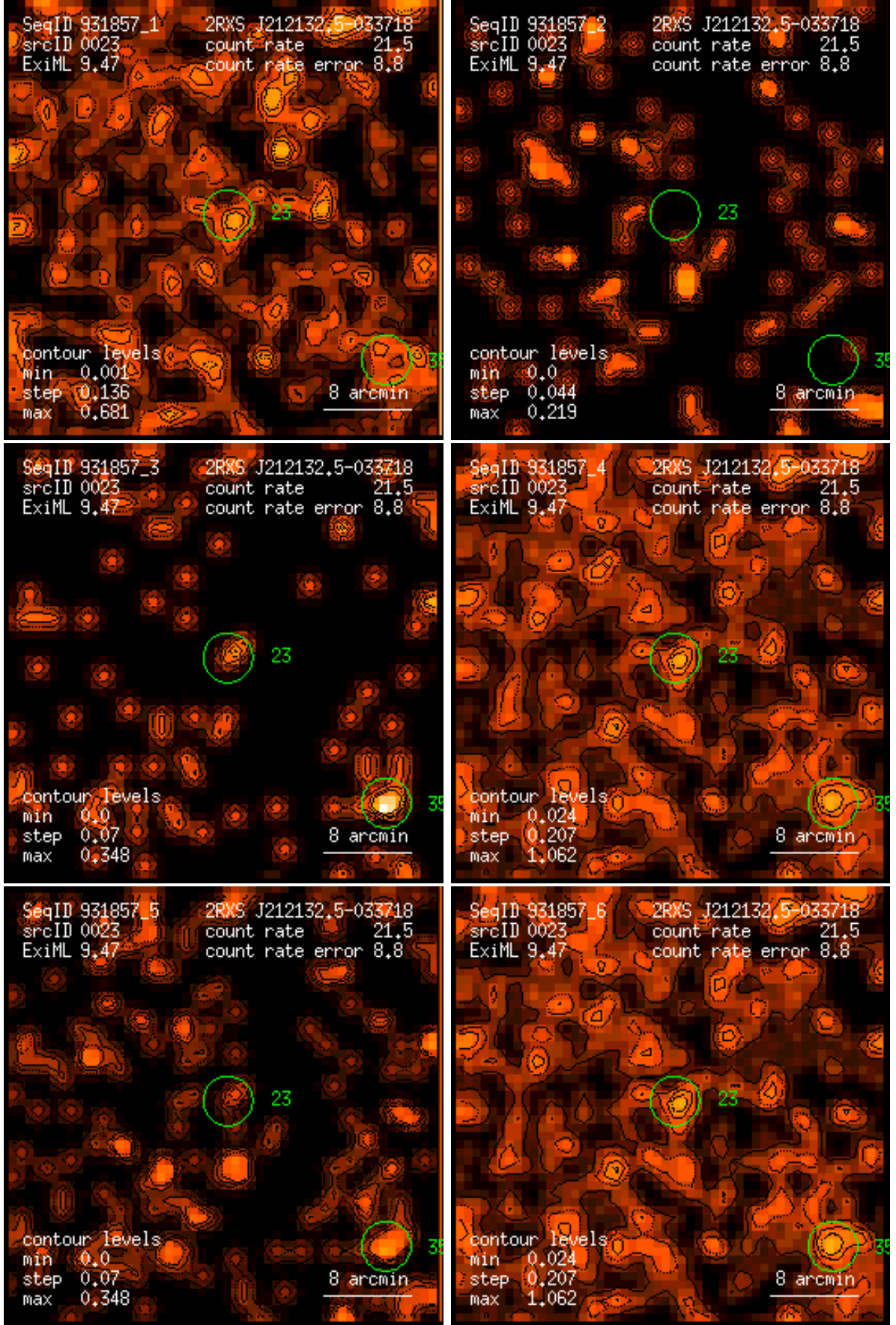
Figure 23: RASS 931857: detection 0023: band rate images, Gaussian filter: (1) PSPC channels 11 – 41, (2) 52 – 90, (3) 91 – 201, (4) 11 – 235, (5) 52 – 201, (6) 11 – 201. Broad band rates in counts/ks. Band rate contour levels in counts/ks/arcmin 2 .
