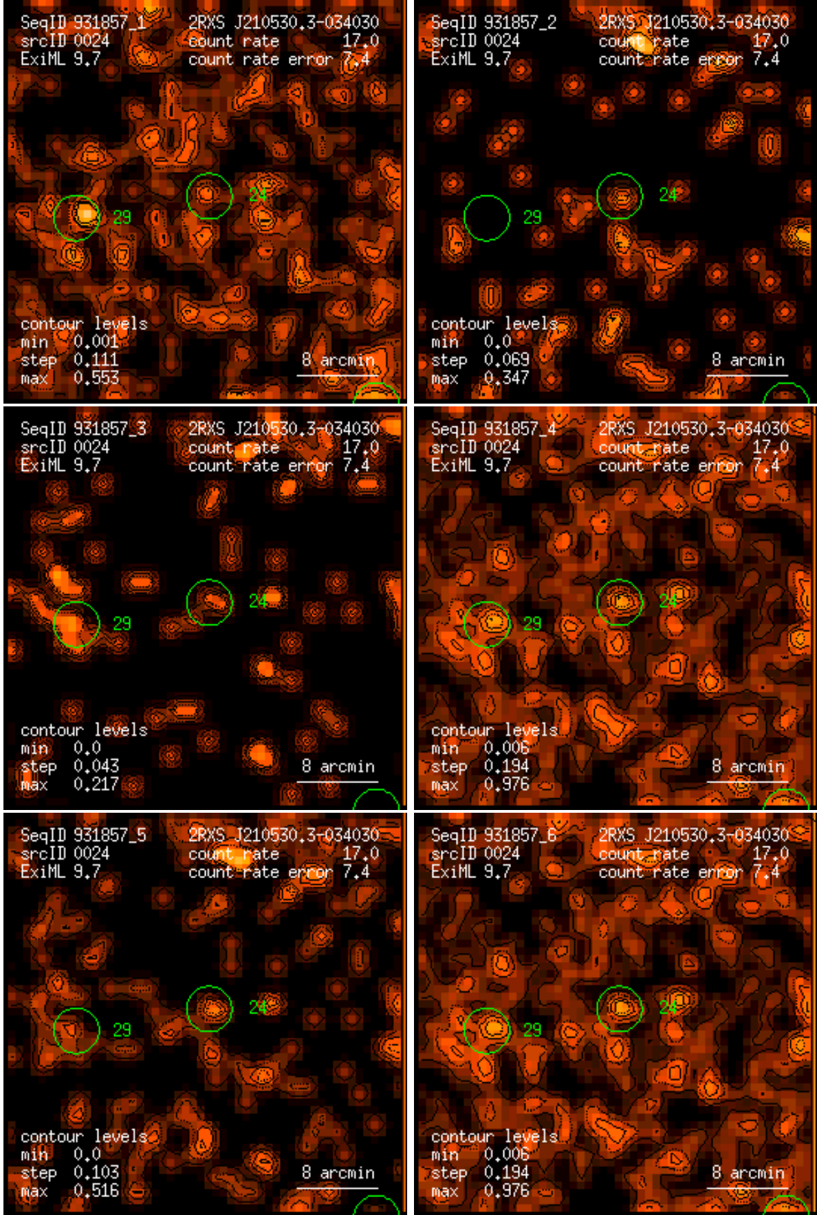
Figure 24: RASS 931857: detection 0024: band rate images, Gaussian filter: (1) PSPC channels 11 – 41, (2) 52 – 90, (3) 91 – 201, (4) 11 – 235, (5) 52 – 201, (6) 11 – 201. Broad band rates in counts/ks. Band rate contour levels in counts/ks/arcmin 2 .
