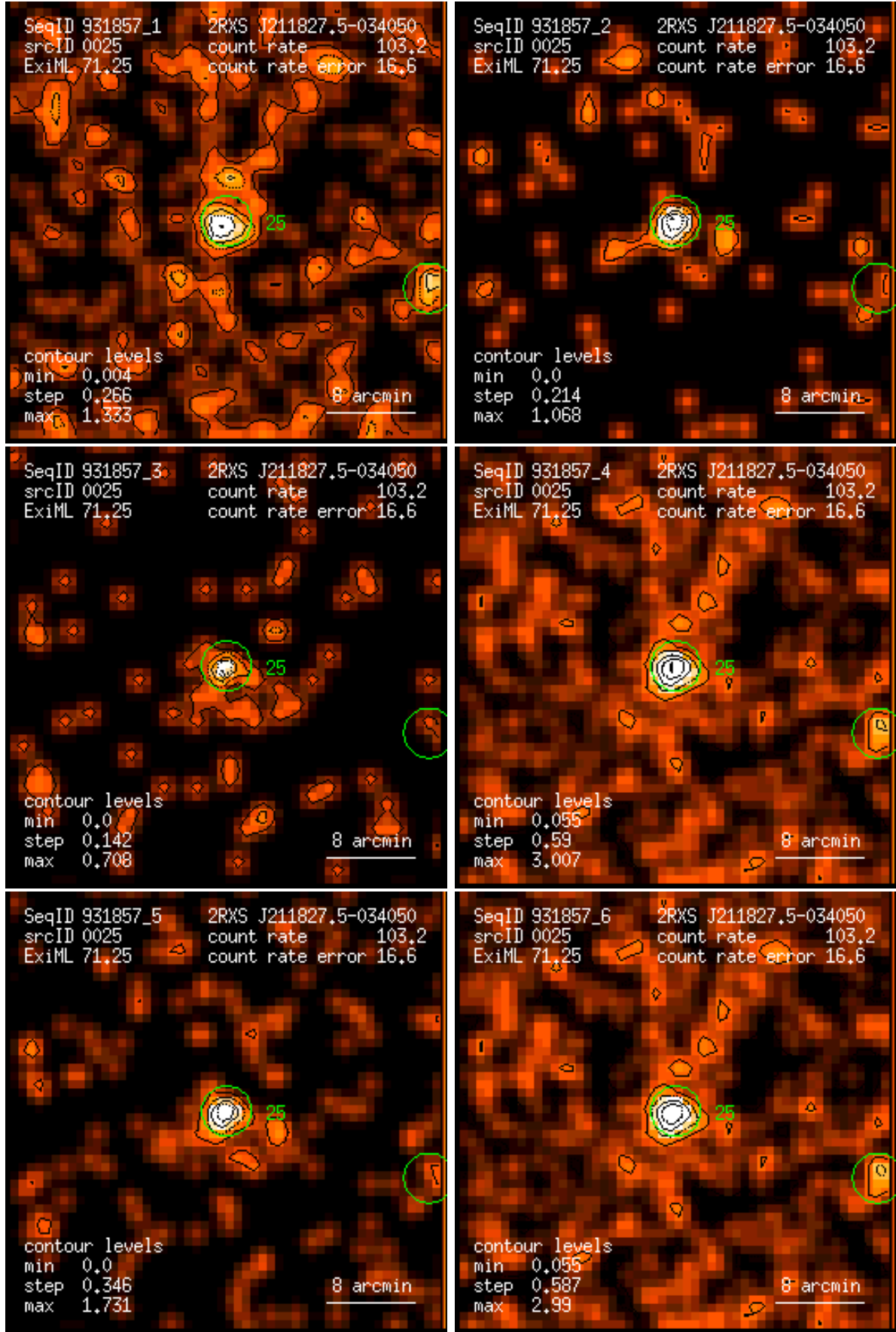
Figure 25: RASS 931857: detection 0025: band rate images, Gaussian filter: (1) PSPC channels 11 – 41, (2) 52 – 90, (3) 91 – 201, (4) 11 – 235, (5) 52 – 201, (6) 11 – 201. Broad band rates in counts/ks. Band rate contour levels in counts/ks/arcmin 2 .
