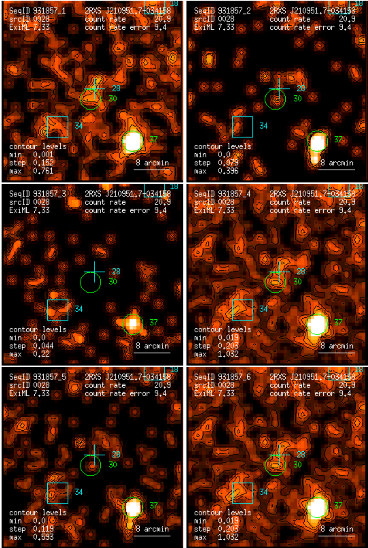
Figure 28: RASS 931857: detection 0028: band rate images, Gaussian filter: (1) PSPC channels 11 – 41, (2) 52 – 90, (3) 91 – 201, (4) 11 – 235, (5) 52 – 201, (6) 11 – 201. Broad band rates in counts/ks. Band rate contour levels in counts/ks/arcmin 2 .
