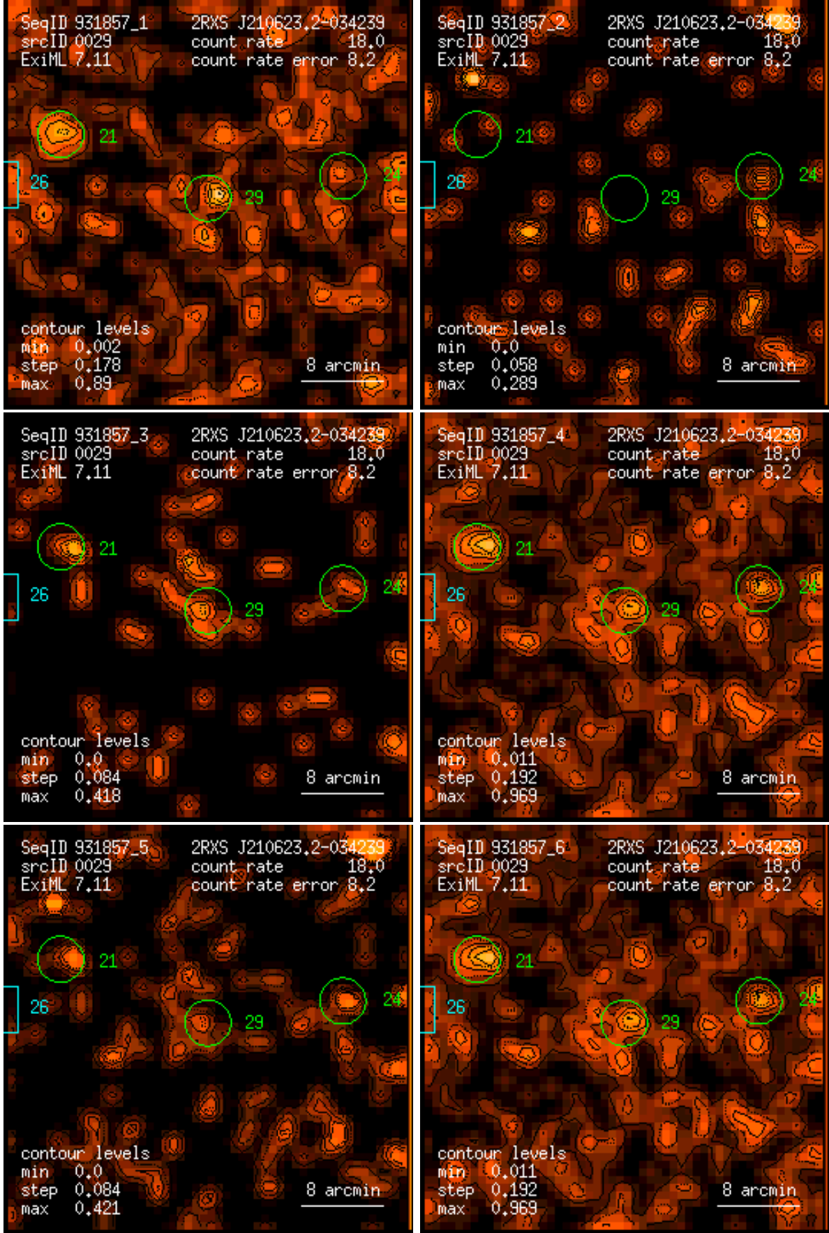
Figure 29: RASS 931857: detection 0029: band rate images, Gaussian filter: (1) PSPC channels 11 – 41, (2) 52 – 90, (3) 91 – 201, (4) 11 – 235, (5) 52 – 201, (6) 11 – 201. Broad band rates in counts/ks. Band rate contour levels in counts/ks/arcmin 2 .
