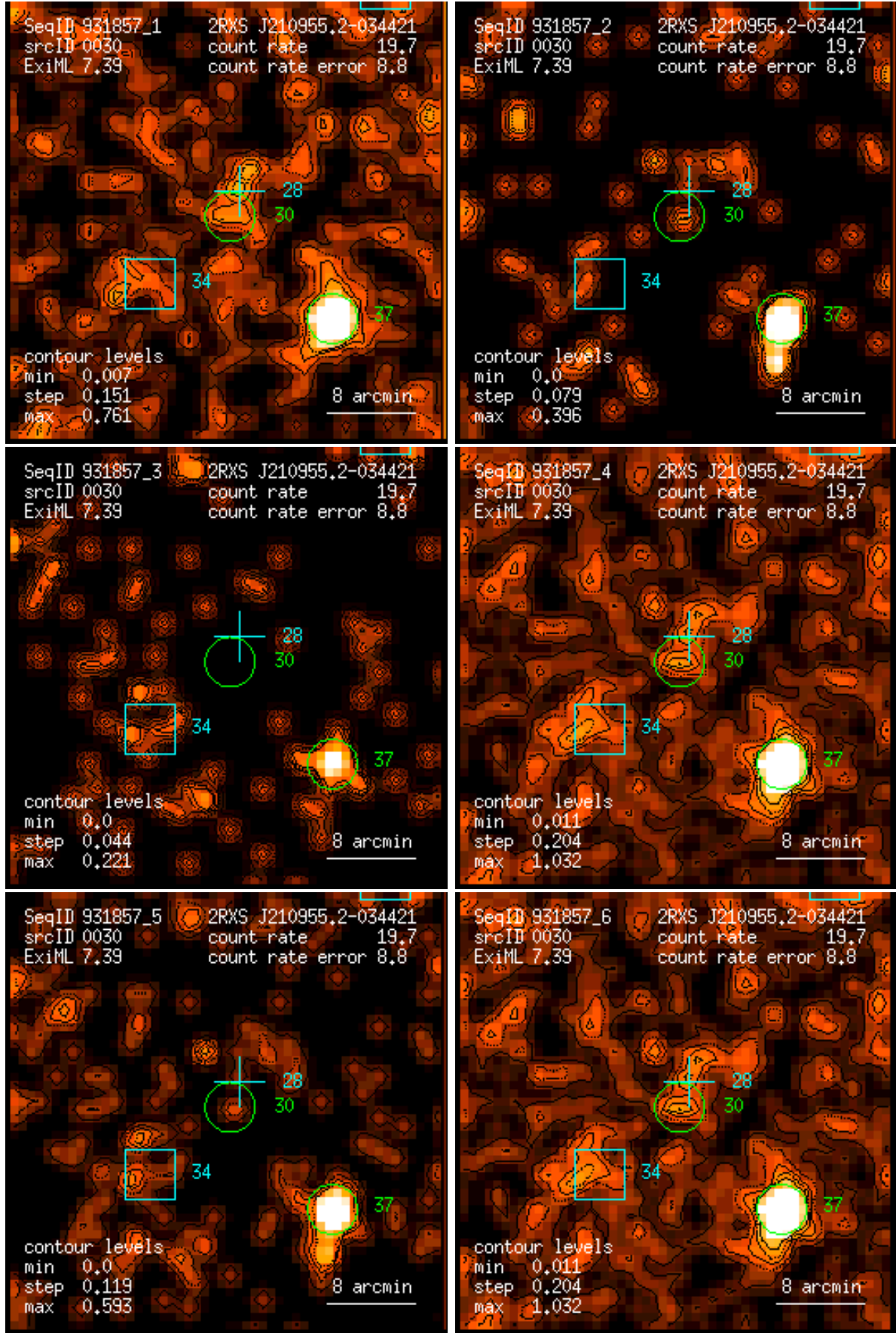
Figure 30: RASS 931857: detection 0030: band rate images, Gaussian filter: (1) PSPC channels 11 – 41, (2) 52 – 90, (3) 91 – 201, (4) 11 – 235, (5) 52 – 201, (6) 11 – 201. Broad band rates in counts/ks. Band rate contour levels in counts/ks/arcmin 2 .
