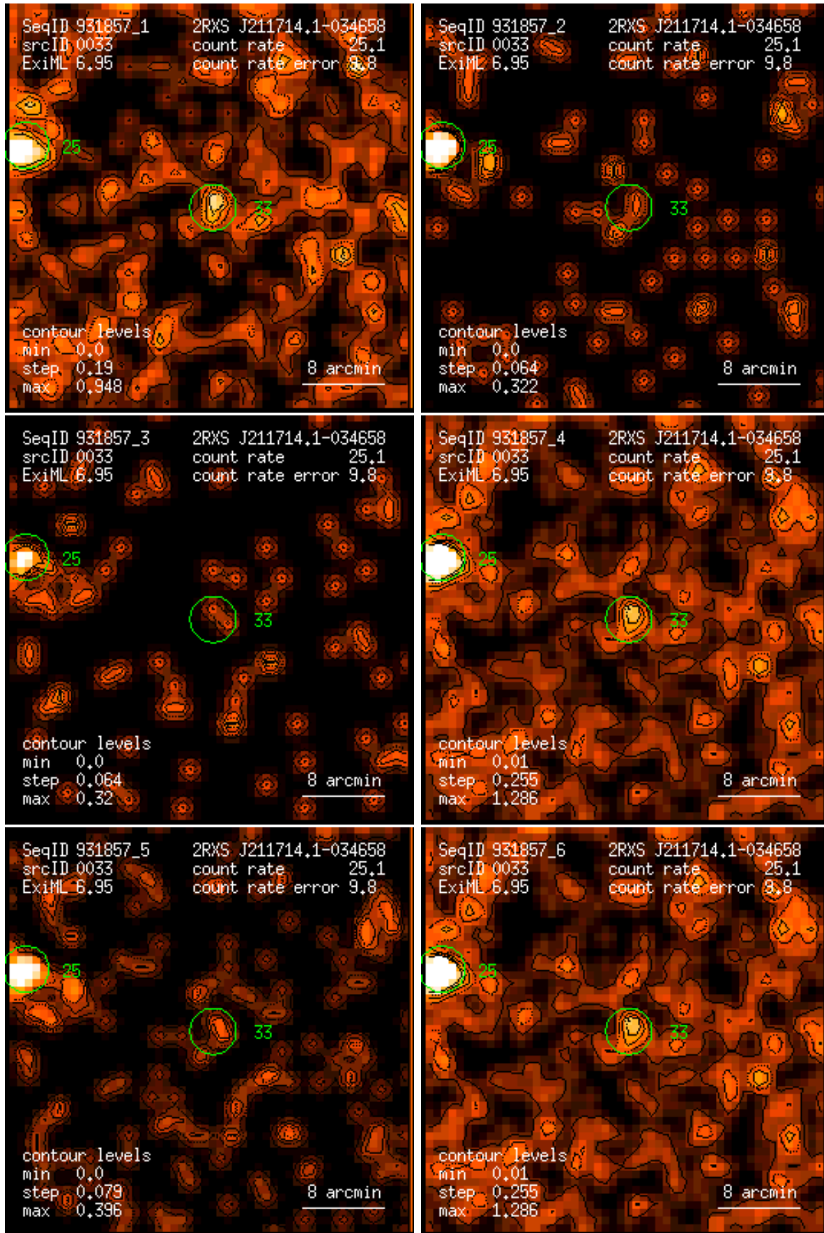
Figure 33: RASS 931857: detection 0033: band rate images, Gaussian filter: (1) PSPC channels 11 – 41, (2) 52 – 90, (3) 91 – 201, (4) 11 – 235, (5) 52 – 201, (6) 11 – 201. Broad band rates in counts/ks. Band rate contour levels in counts/ks/arcmin 2 .
