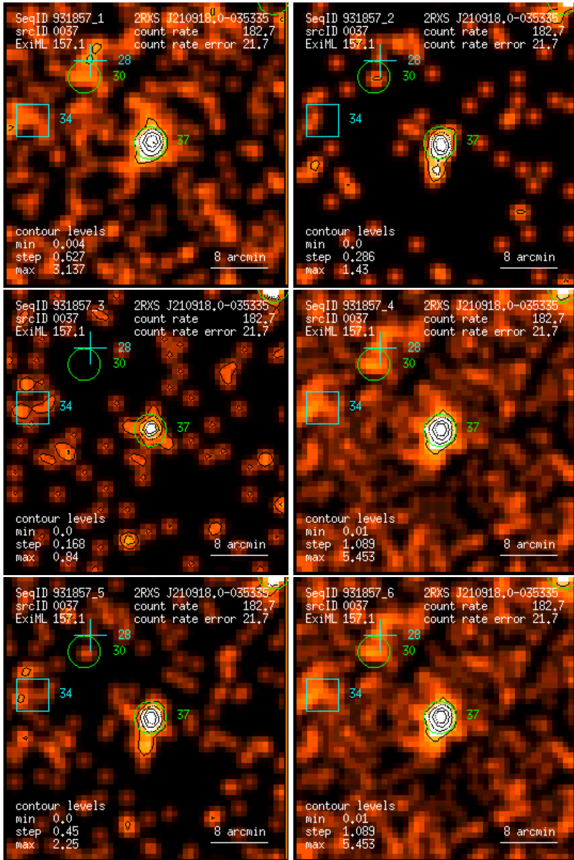
Figure 37: RASS 931857: detection 0037: band rate images, Gaussian filter: (1) PSPC channels 11 – 41, (2) 52 – 90, (3) 91 – 201, (4) 11 – 235, (5) 52 – 201, (6) 11 – 201. Broad band rates in counts/ks. Band rate contour levels in counts/ks/arcmin 2 .
