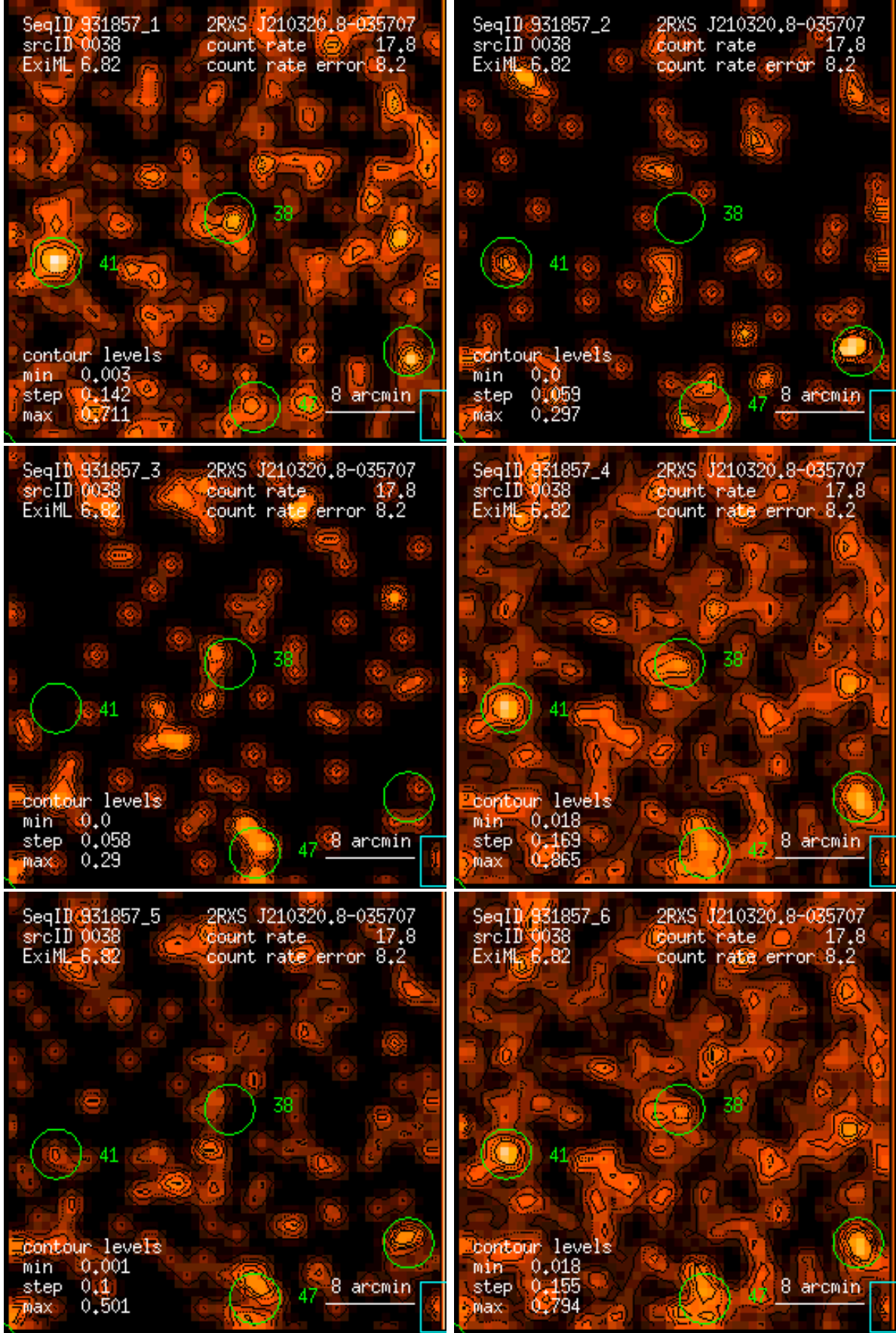
Figure 38: RASS 931857: detection 0038: band rate images, Gaussian filter: (1) PSPC channels 11 – 41, (2) 52 – 90, (3) 91 – 201, (4) 11 – 235, (5) 52 – 201, (6) 11 – 201. Broad band rates in counts/ks. Band rate contour levels in counts/ks/arcmin 2 .
