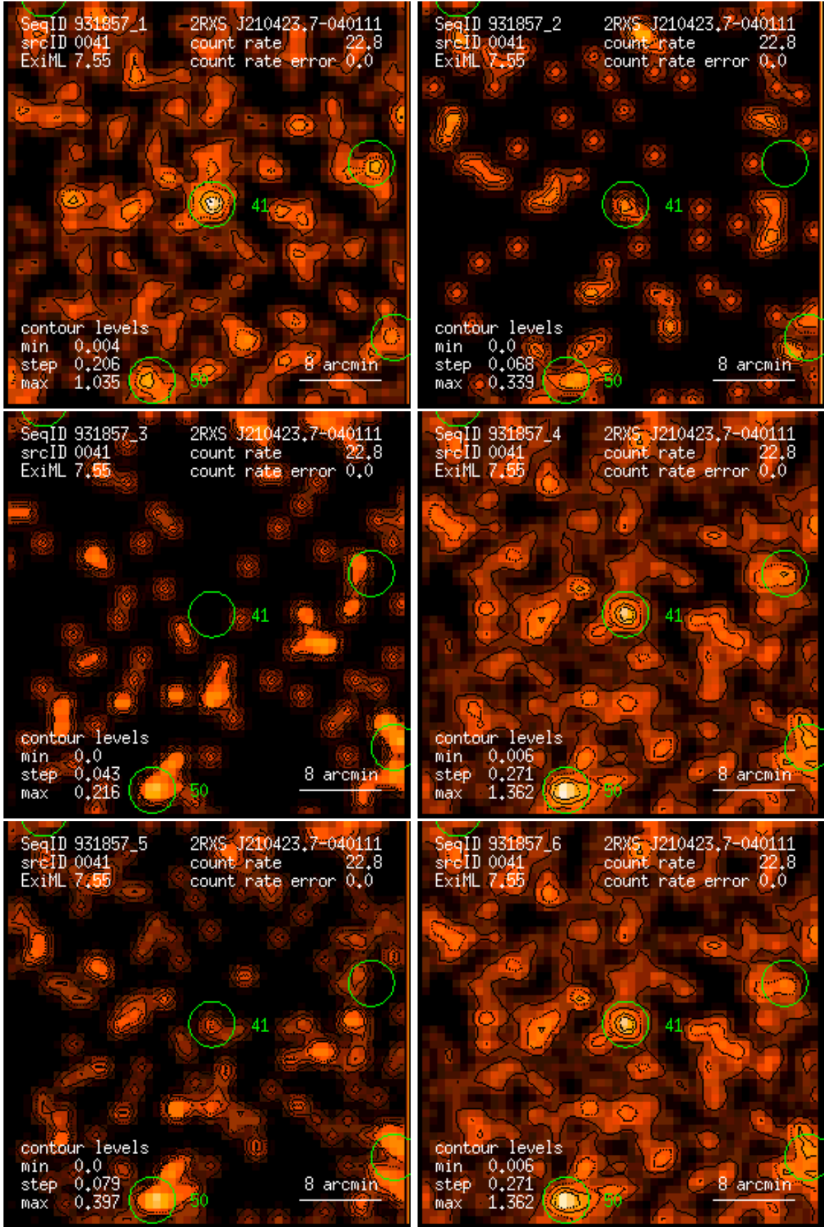
Figure 41: RASS 931857: detection 0041: band rate images, Gaussian filter: (1) PSPC channels 11 – 41, (2) 52 – 90, (3) 91 – 201, (4) 11 – 235, (5) 52 – 201, (6) 11 – 201. Broad band rates in counts/ks. Band rate contour levels in counts/ks/arcmin 2 .
