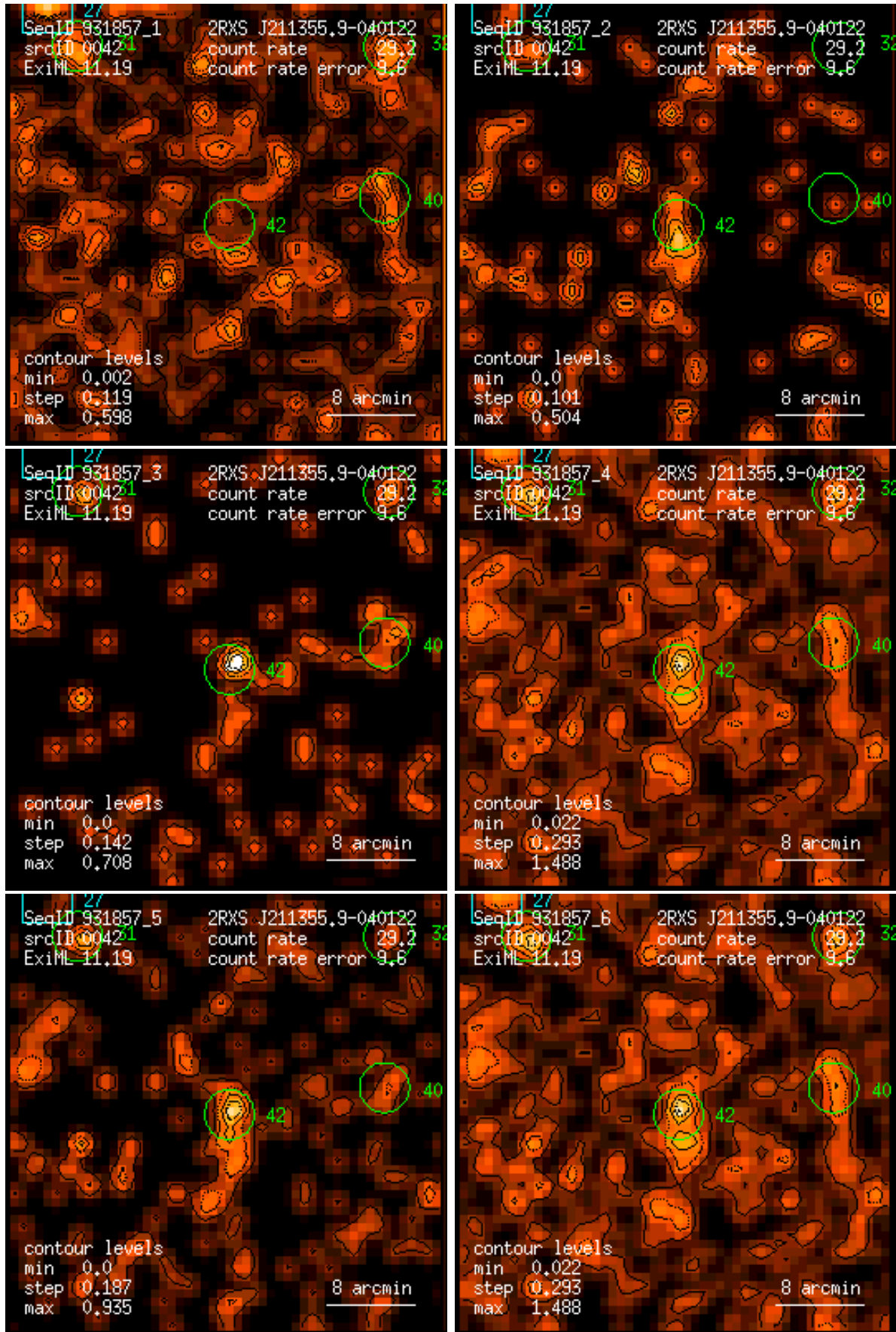
Figure 42: RASS 931857: detection 0042: band rate images, Gaussian filter: (1) PSPC channels 11 – 41, (2) 52 – 90, (3) 91 – 201, (4) 11 – 235, (5) 52 – 201, (6) 11 – 201. Broad band rates in counts/ks. Band rate contour levels in counts/ks/arcmin 2 .
