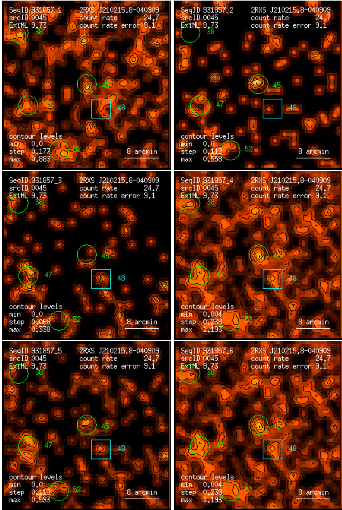
Figure 45: RASS 931857: detection 0045: band rate images, Gaussian filter: (1) PSPC channels 11 – 41, (2) 52 – 90, (3) 91 – 201, (4) 11 – 235, (5) 52 – 201, (6) 11 – 201. Broad band rates in counts/ks. Band rate contour levels in counts/ks/arcmin 2 .
