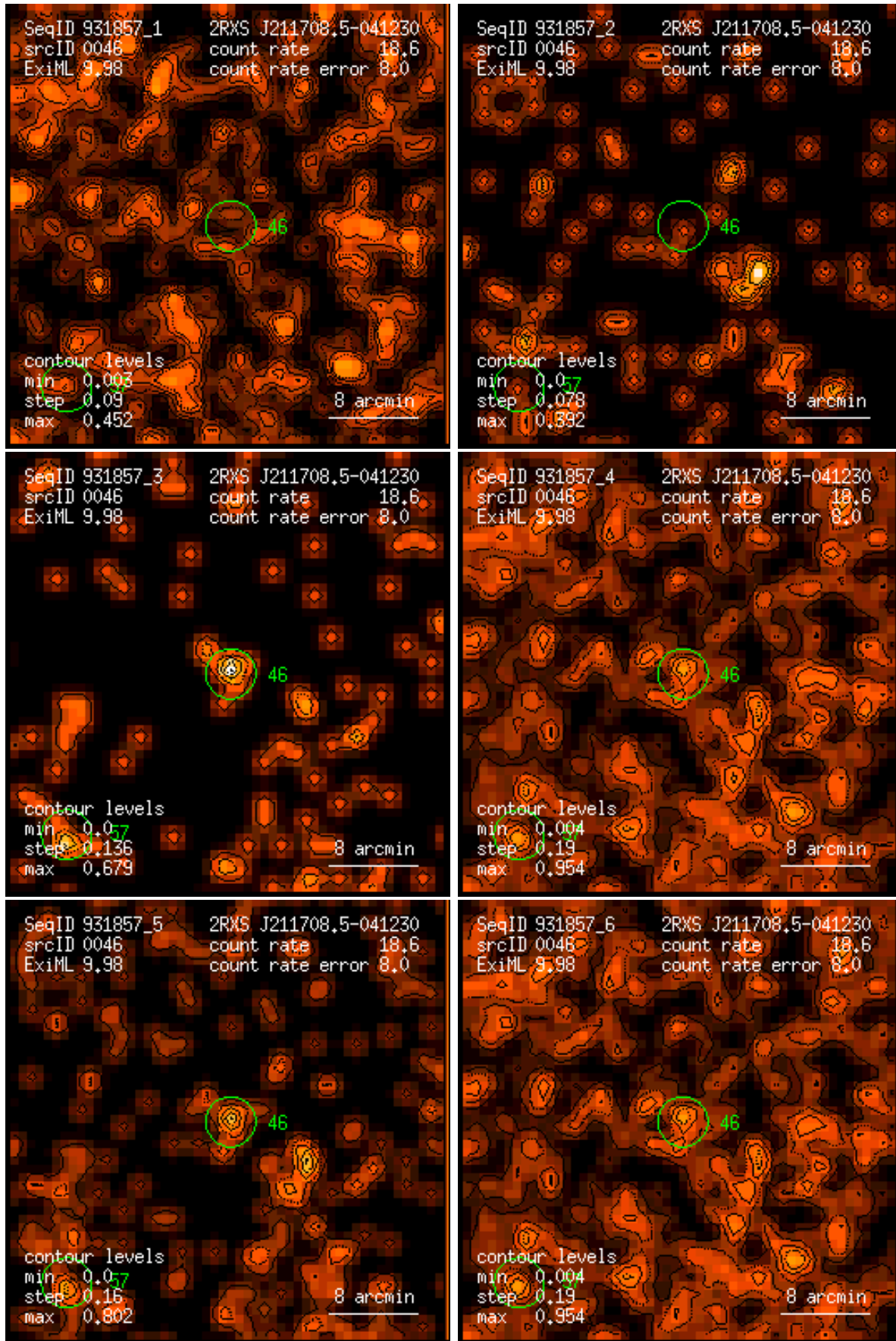
Figure 46: RASS 931857: detection 0046: band rate images, Gaussian filter: (1) PSPC channels 11 – 41, (2) 52 – 90, (3) 91 – 201, (4) 11 – 235, (5) 52 – 201, (6) 11 – 201. Broad band rates in counts/ks. Band rate contour levels in counts/ks/arcmin 2 .
