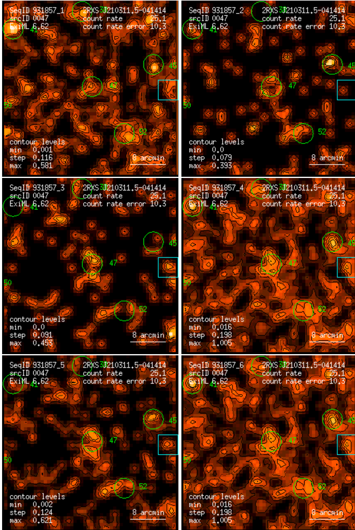
Figure 47: RASS 931857: detection 0047: band rate images, Gaussian filter: (1) PSPC channels 11 – 41, (2) 52 – 90, (3) 91 – 201, (4) 11 – 235, (5) 52 – 201, (6) 11 – 201. Broad band rates in counts/ks. Band rate contour levels in counts/ks/arcmin 2 .
