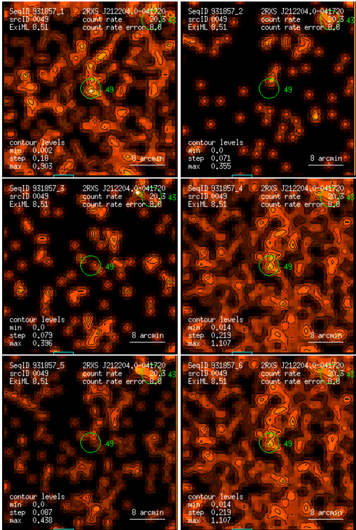
Figure 49: RASS 931857: detection 0049: band rate images, Gaussian filter: (1) PSPC channels 11 – 41, (2) 52 – 90, (3) 91 – 201, (4) 11 – 235, (5) 52 – 201, (6) 11 – 201. Broad band rates in counts/ks. Band rate contour levels in counts/ks/arcmin 2 .
