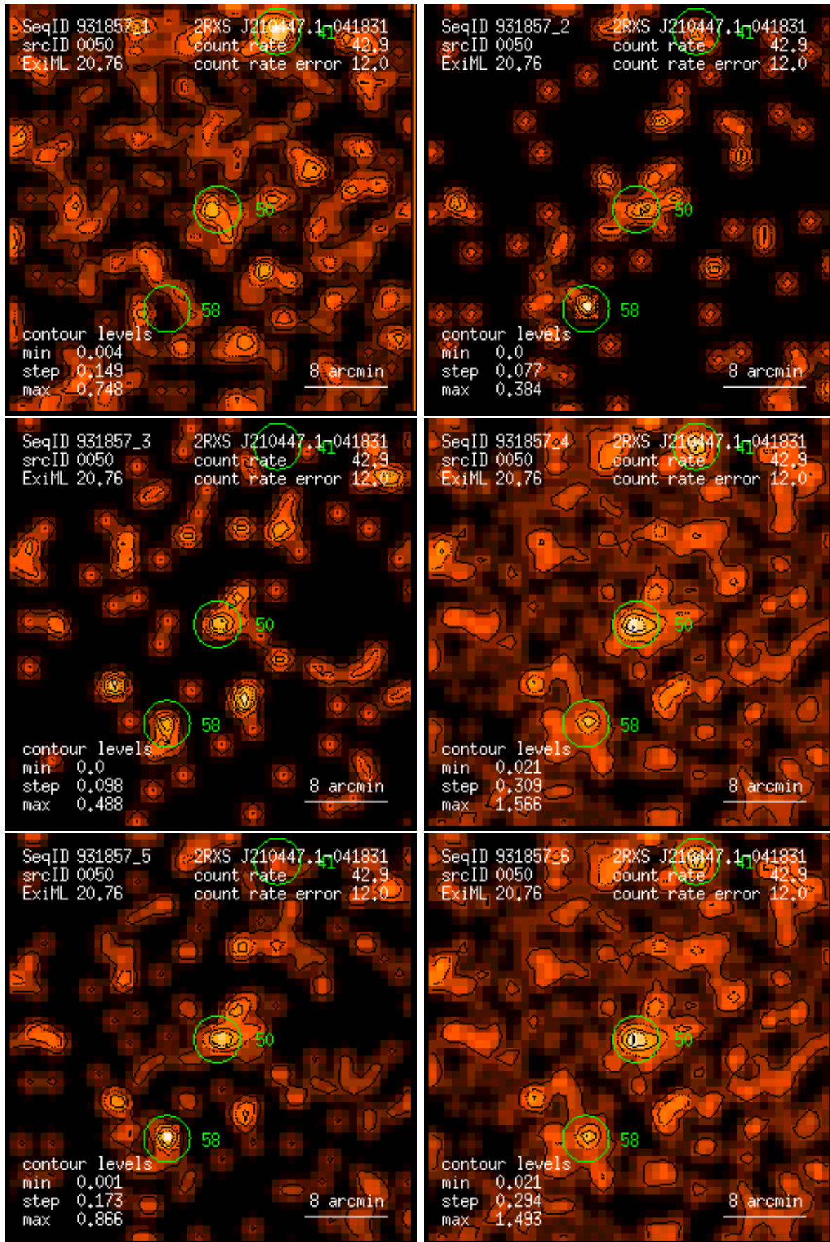
Figure 50: RASS 931857: detection 0050: band rate images, Gaussian filter: (1) PSPC channels 11 – 41, (2) 52 – 90, (3) 91 – 201, (4) 11 – 235, (5) 52 – 201, (6) 11 – 201. Broad band rates in counts/ks. Band rate contour levels in counts/ks/arcmin 2 .
