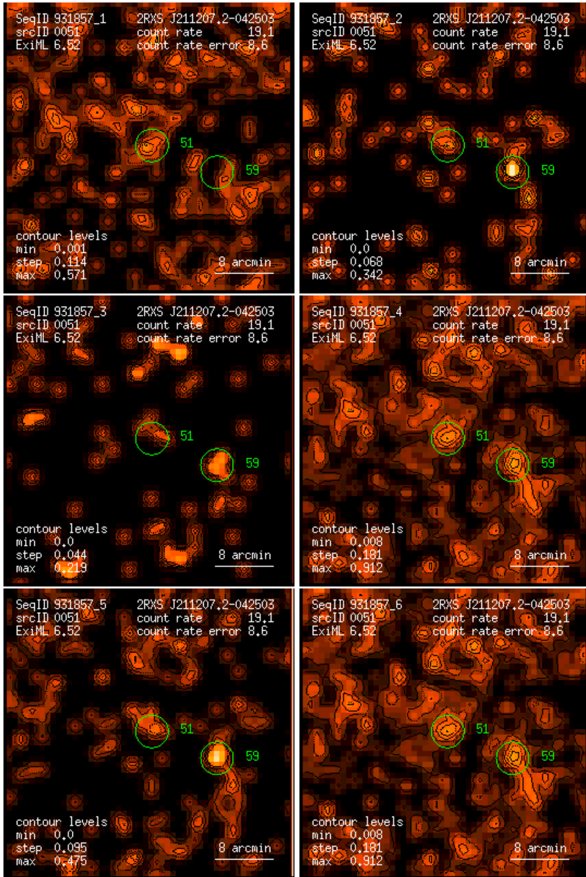
Figure 51: RASS 931857: detection 0051: band rate images, Gaussian filter: (1) PSPC channels 11 – 41, (2) 52 – 90, (3) 91 – 201, (4) 11 – 235, (5) 52 – 201, (6) 11 – 201. Broad band rates in counts/ks. Band rate contour levels in counts/ks/arcmin 2 .
