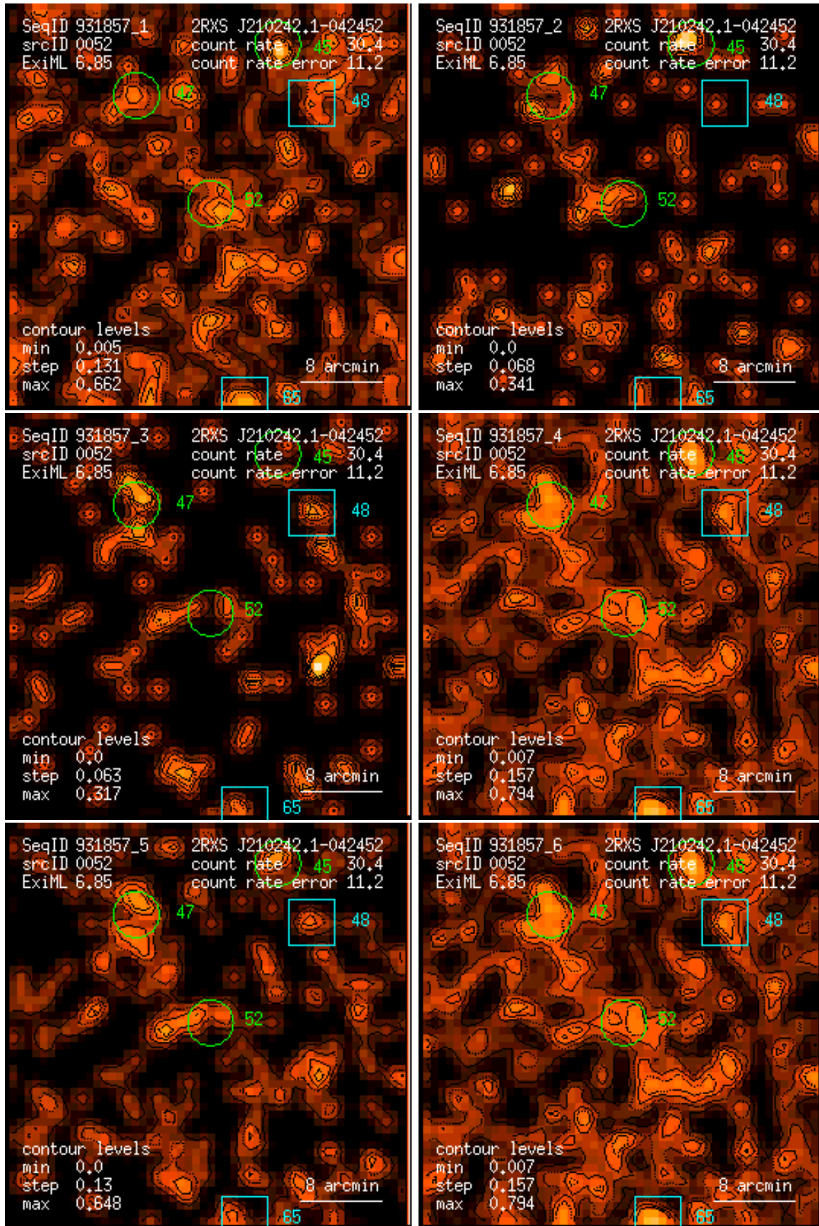
Figure 52: RASS 931857: detection 0052: band rate images, Gaussian filter: (1) PSPC channels 11 – 41, (2) 52 – 90, (3) 91 – 201, (4) 11 – 235, (5) 52 – 201, (6) 11 – 201. Broad band rates in counts/ks. Band rate contour levels in counts/ks/arcmin 2 .
