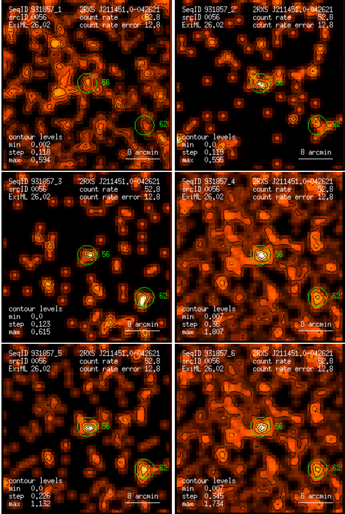
Figure 56: RASS 931857: detection 0056: band rate images, Gaussian filter: (1) PSPP channels 11 – 41, (2) 52 – 90, (3) 91 – 201, (4) 11 – 235, (5) 52 – 201, (6) 11 – 201. Broad band rates in counts/ks. Band rate contour levels in counts/ks/arcmin 2 .
