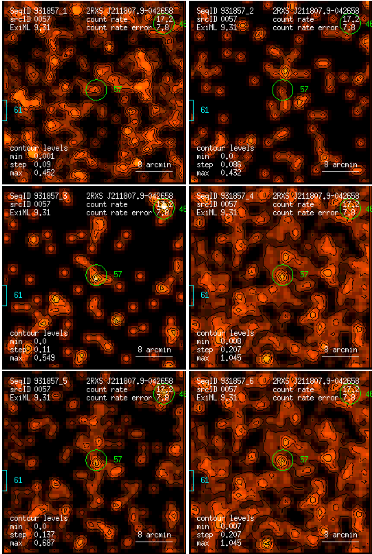
Figure 57: RASS 931857: detection 0057: band rate images, Gaussian filter: (1) PSPC channels 11 – 41, (2) 52 – 90, (3) 91 – 201, (4) 11 – 235, (5) 52 – 201, (6) 11 – 201. Broad band rates in counts/ks. Band rate contour levels in counts/ks/arcmin 2 .
