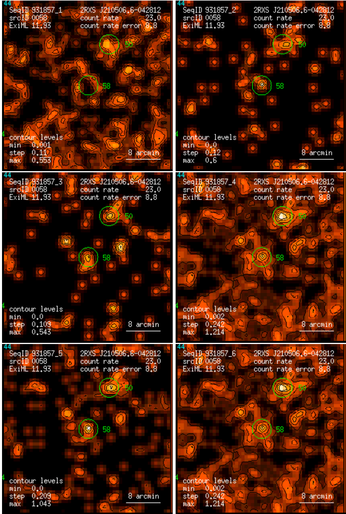
Figure 58: RASS 931857: detection 0058: band rate images, Gaussian filter: (1) PSPC channels 11 – 41, (2) 52 – 90, (3) 91 – 201, (4) 11 – 235, (5) 52 – 201, (6) 11 – 201. Broad band rates in counts/ks. Band rate contour levels in counts/ks/arcmin 2 .
