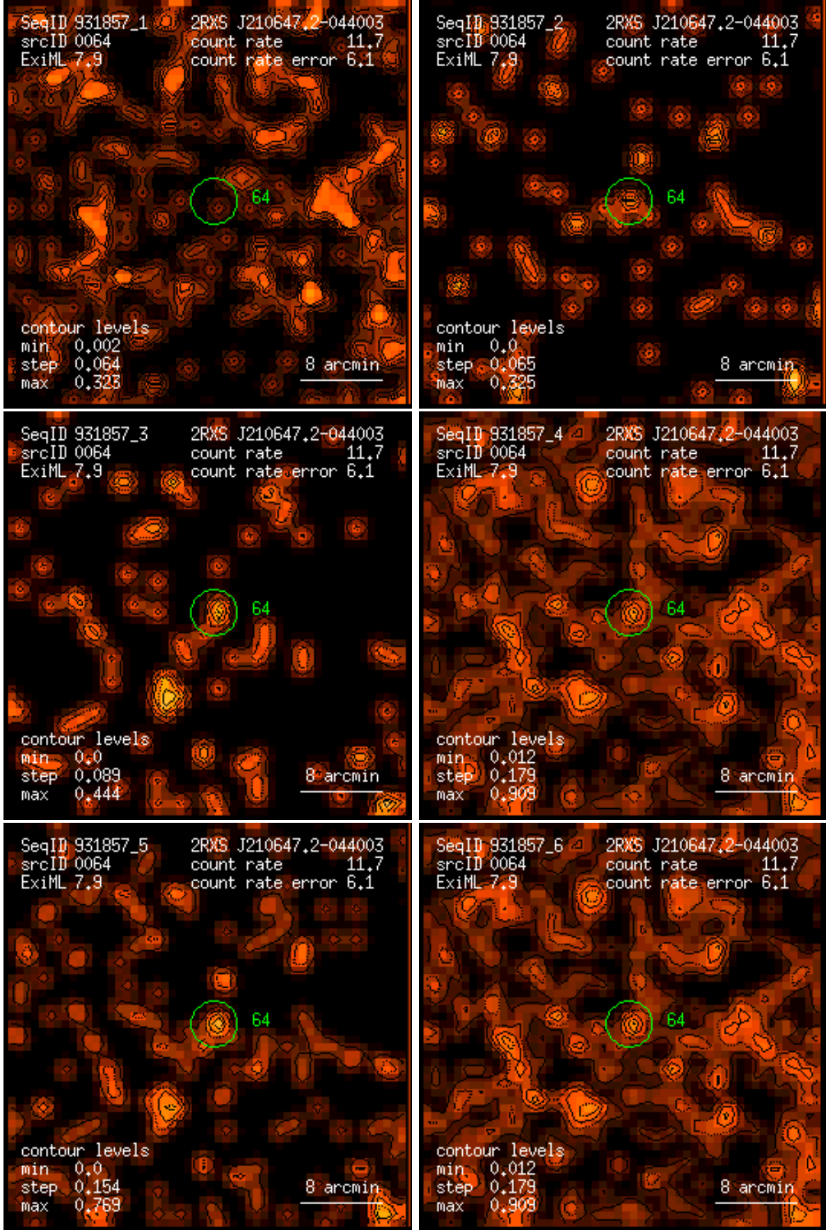
Figure 64: RASS 931857: detection 0064: band rate images, Gaussian filter: (1) PSPC channels 11 – 41, (2) 52 – 90, (3) 91 – 201, (4) 11 – 235, (5) 52 – 201, (6) 11 – 201. Broad band rates in counts/ks. Band rate contour levels in counts/ks/arcmin 2 .
