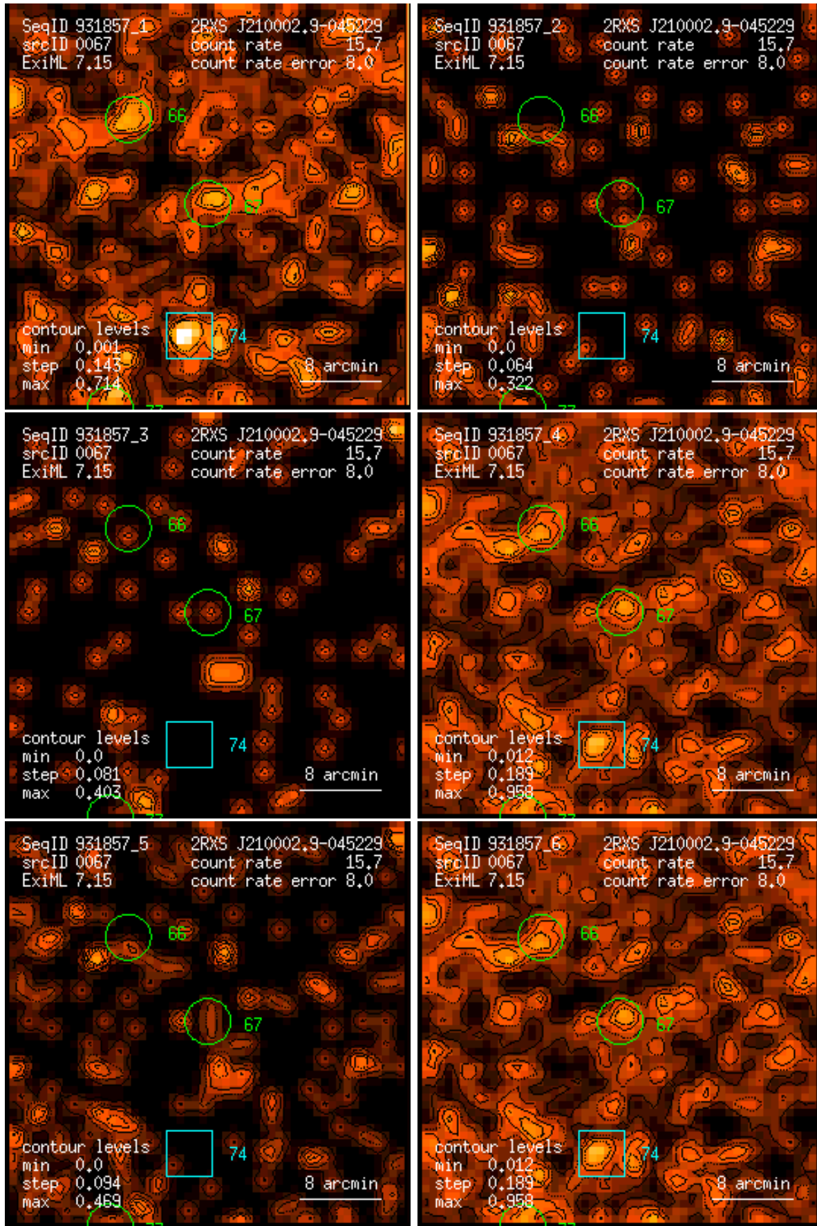
Figure 67: RASS 931857: detection 0067: band rate images, Gaussian filter: (1) PSPC channels 11 – 41, (2) 52 – 90, (3) 91 – 201, (4) 11 – 235, (5) 52 – 201, (6) 11 – 201. Broad band rates in counts/ks. Band rate contour levels in counts/ks/arcmin 2 .
