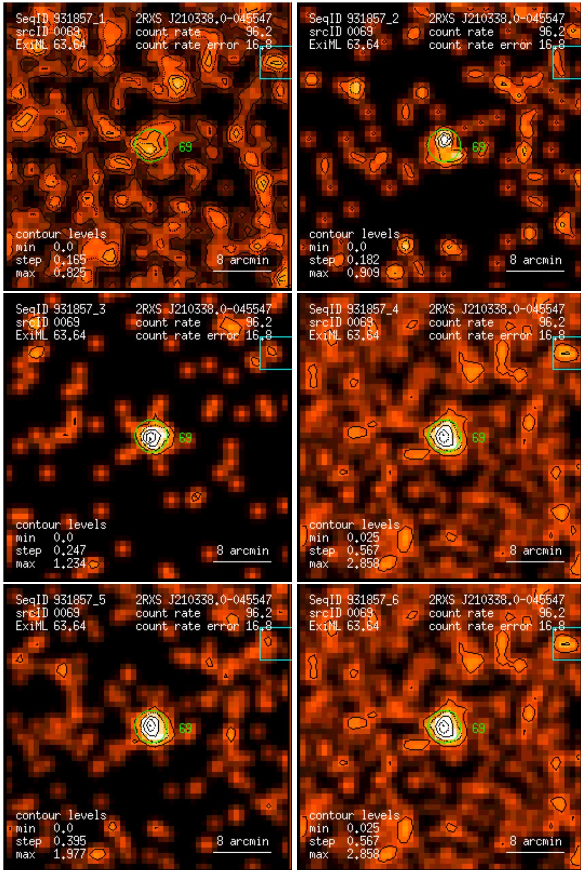
Figure 69: RASS 931857: detection 0069: band rate images, Gaussian filter: (1) PSPC channels 11 – 41, (2) 52 – 90, (3) 91 – 201, (4) 11 – 235, (5) 52 – 201, (6) 11 – 201. Broad band rates in counts/ks. Band rate contour levels in counts/ks/arcmin 2 .
