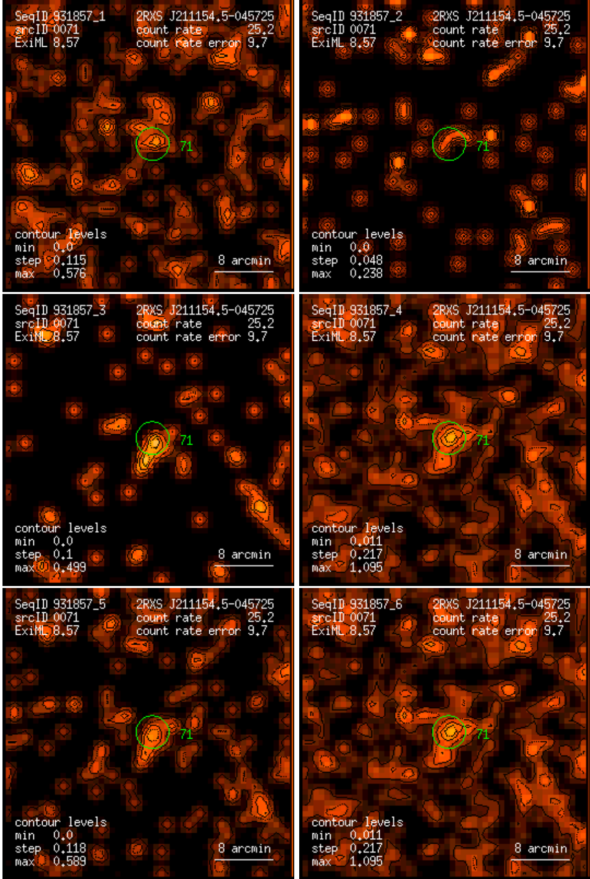
Figure 71: RASS 931857: detection 0071: band rate images, Gaussian filter: (1) PSPC channels 11 – 41, (2) 52 – 90, (3) 91 – 201, (4) 11 – 235, (5) 52 – 201, (6) 11 – 201. Broad band rates in counts/ks. Band rate contour levels in counts/ks/arcmin 2 .
