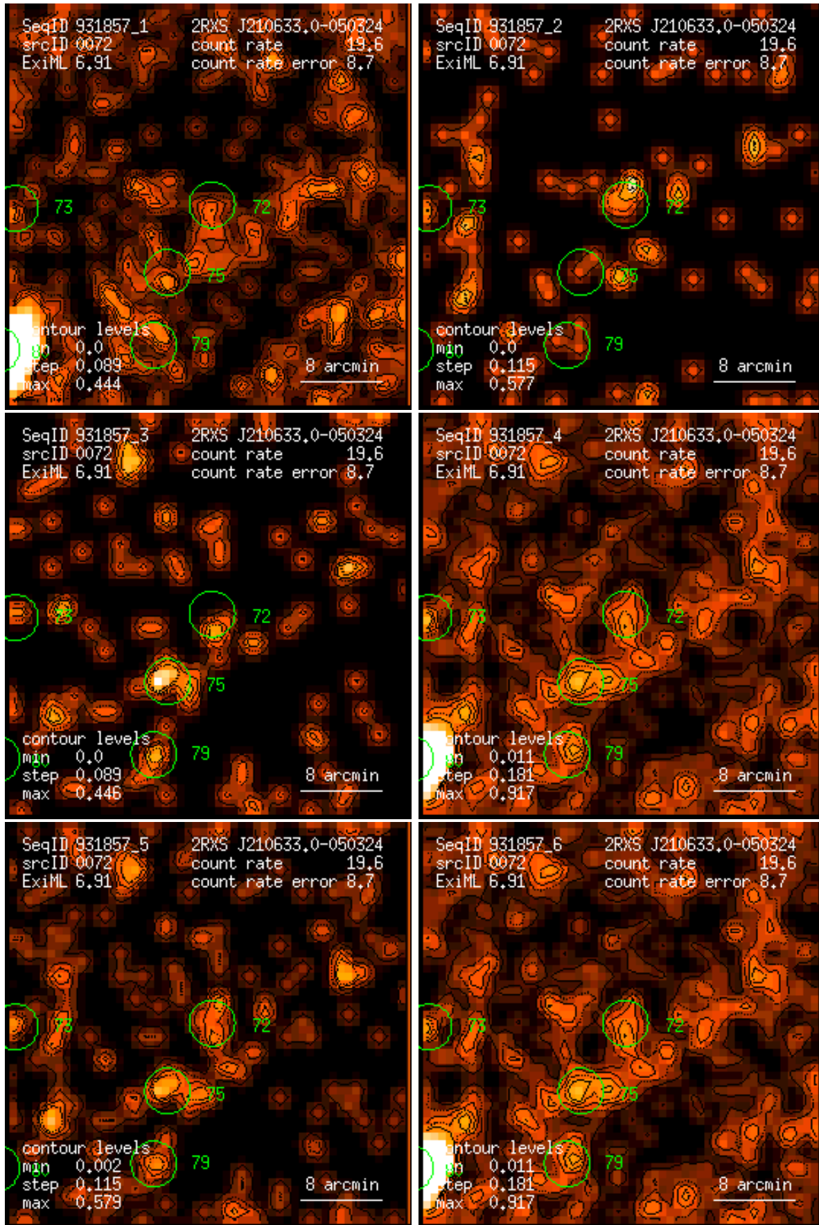
Figure 72: RASS 931857: detection 0072: band rate images, Gaussian filter: (1) PSPC channels 11 – 41, (2) 52 – 90, (3) 91 – 201, (4) 11 – 235, (5) 52 – 201, (6) 11 – 201. Broad band rates in counts/ks. Band rate contour levels in counts/ks/arcmin 2 .
