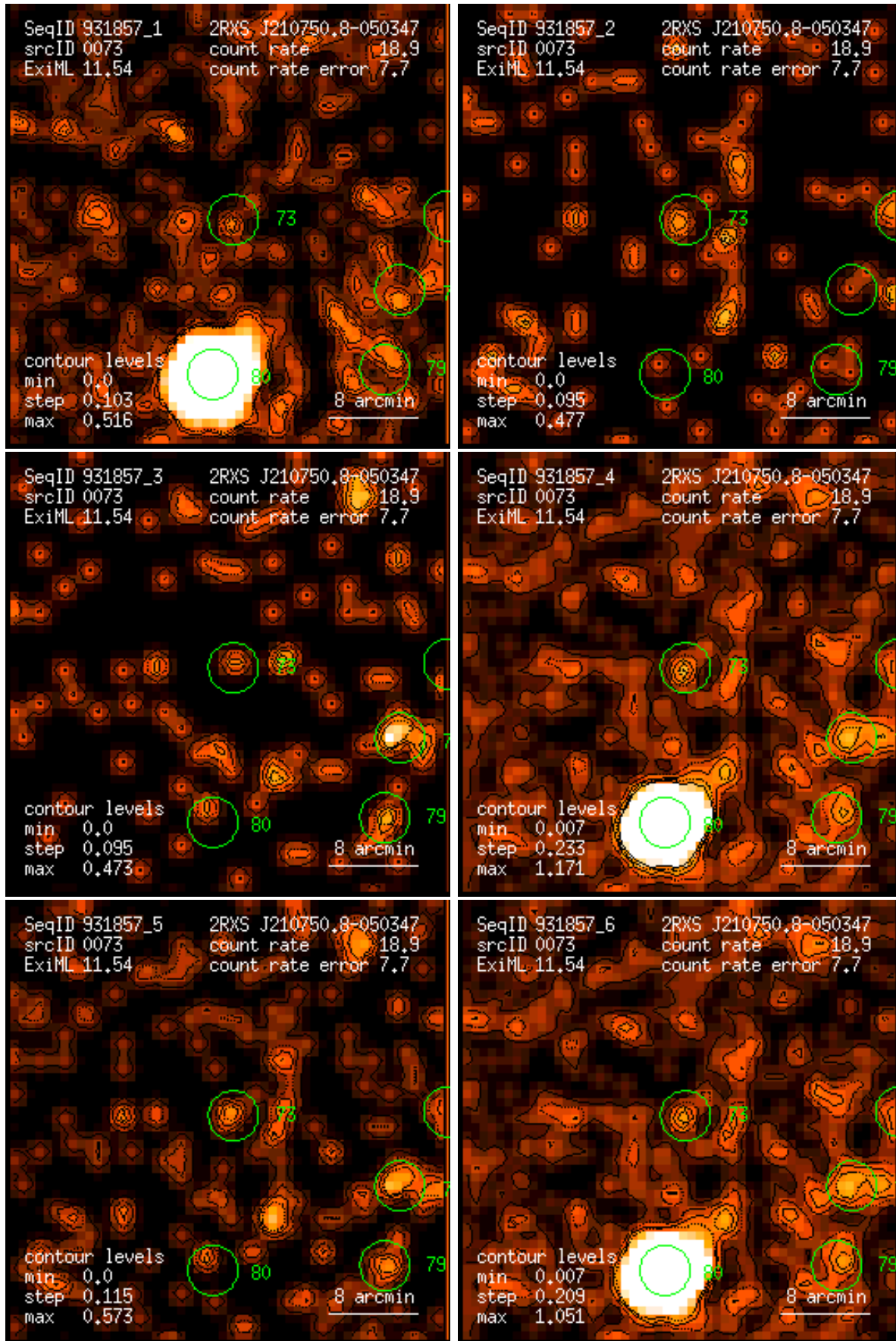
Figure 73: RASS 931857: detection 0073: band rate images, Gaussian filter: (1) PSPC channels 11 – 41, (2) 52 – 90, (3) 91 – 201, (4) 11 – 235, (5) 52 – 201, (6) 11 – 201. Broad band rates in counts/ks. Band rate contour levels in counts/ks/arcmin 2 .
