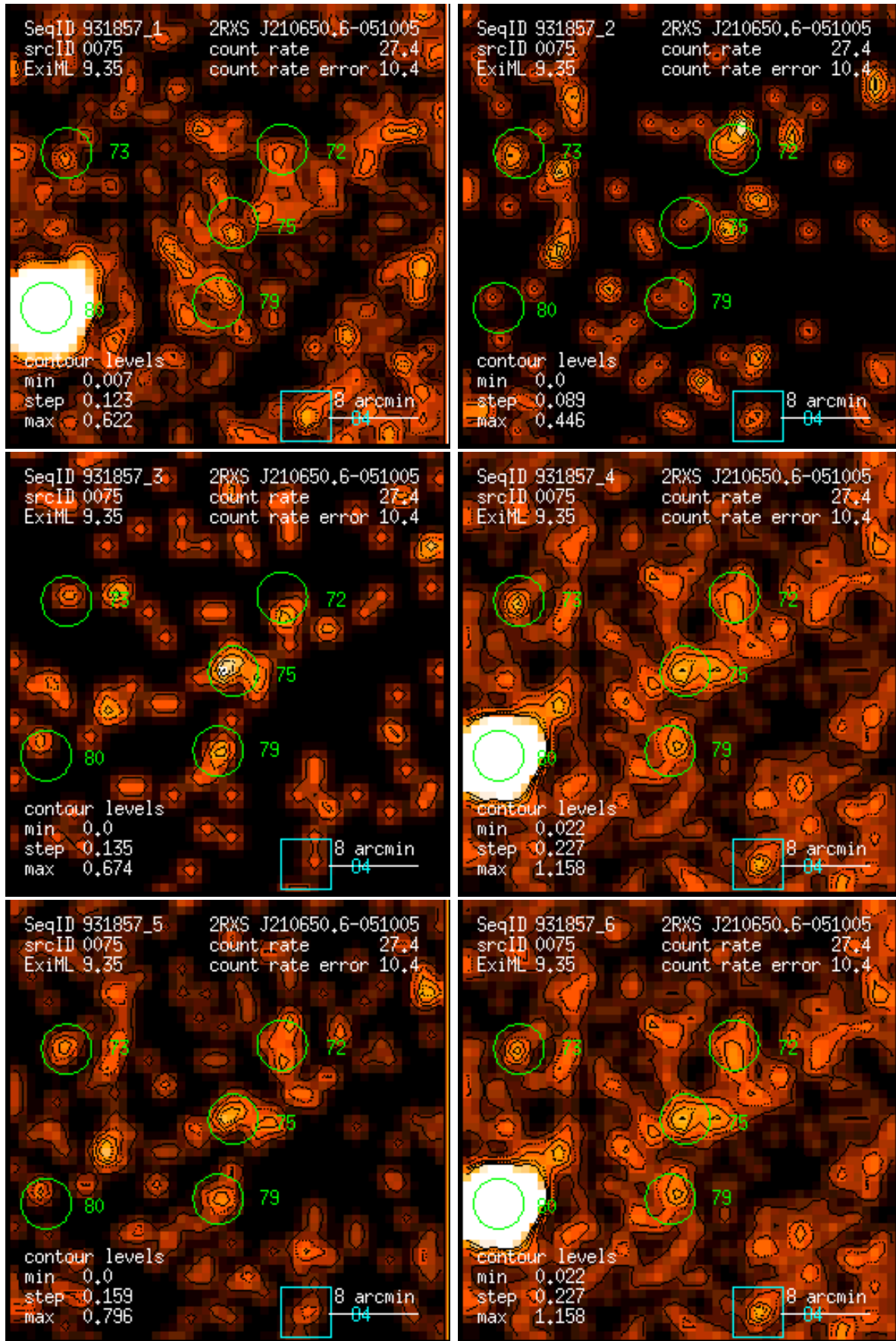
Figure 75: RASS 931857: detection 0075: band rate images, Gaussian filter: (1) PSPC channels 11 – 41, (2) 52 – 90, (3) 91 – 201, (4) 11 – 235, (5) 52 – 201, (6) 11 – 201. Broad band rates in counts/ks. Band rate contour levels in counts/ks/arcmin 2 .
