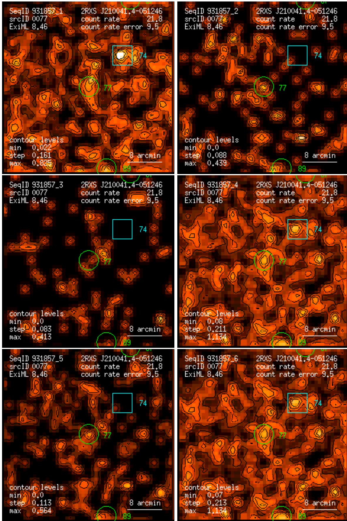
Figure 77: RASS 931857: detection 0077: band rate images, Gaussian filter: (1) PSPC channels 11 – 41, (2) 52 – 90, (3) 91 – 201, (4) 11 – 235, (5) 52 – 201, (6) 11 – 201. Broad band rates in counts/ks. Band rate contour levels in counts/ks/arcmin 2 .
