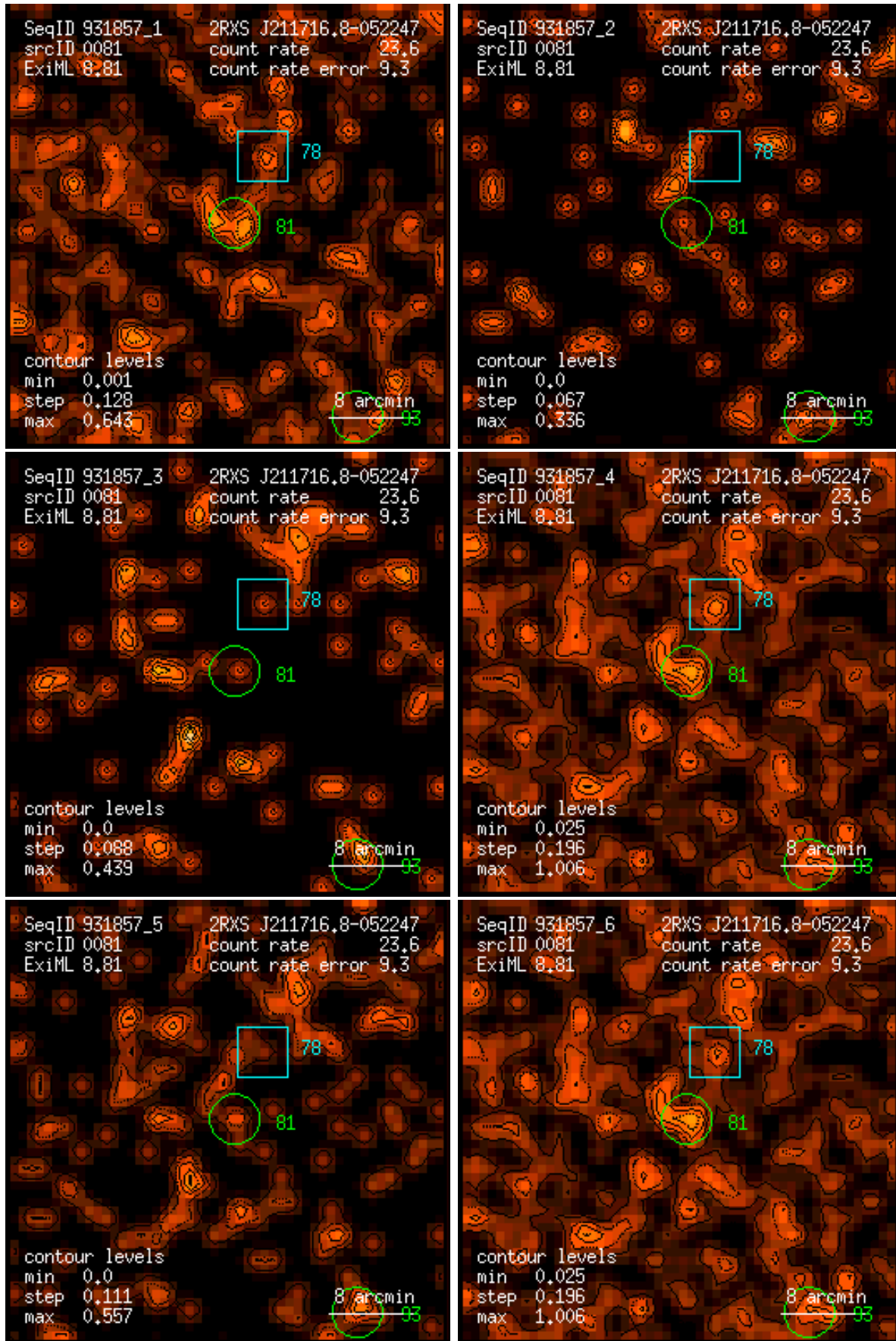
Figure 81: RASS 931857: detection 0081: band rate images, Gaussian filter: (1) PSPC channels 11 – 41, (2) 52 – 90, (3) 91 – 201, (4) 11 – 235, (5) 52 – 201, (6) 11 – 201. Broad band rates in counts/ks. Band rate contour levels in counts/ks/arcmin 2 .
