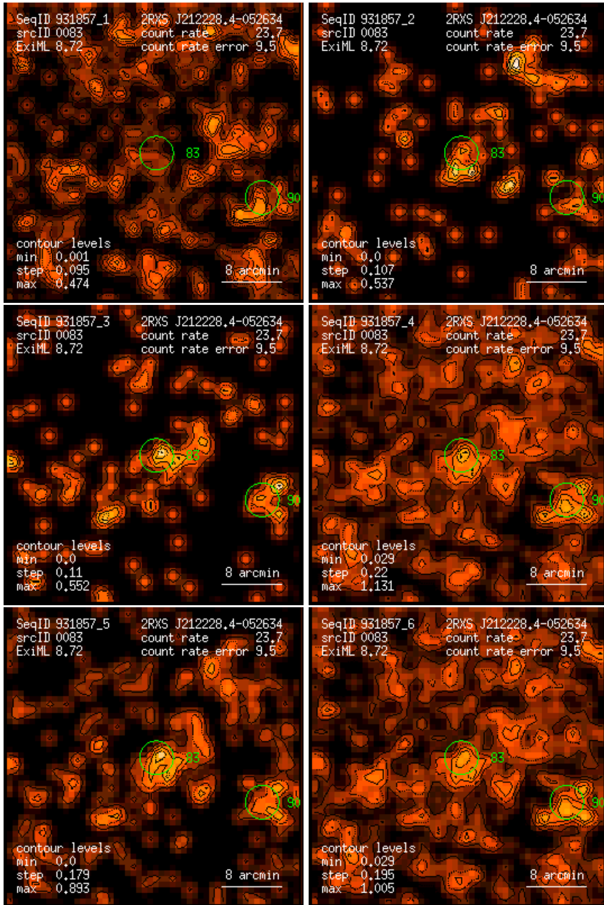
Figure 83: RASS 931857: detection 0083: band rate images, Gaussian filter: (1) PSPC channels 11 – 41, (2) 52 – 90, (3) 91 – 201, (4) 11 – 235, (5) 52 – 201, (6) 11 – 201. Broad band rates in counts/ks. Band rate contour levels in counts/ks/arcmin 2 .
