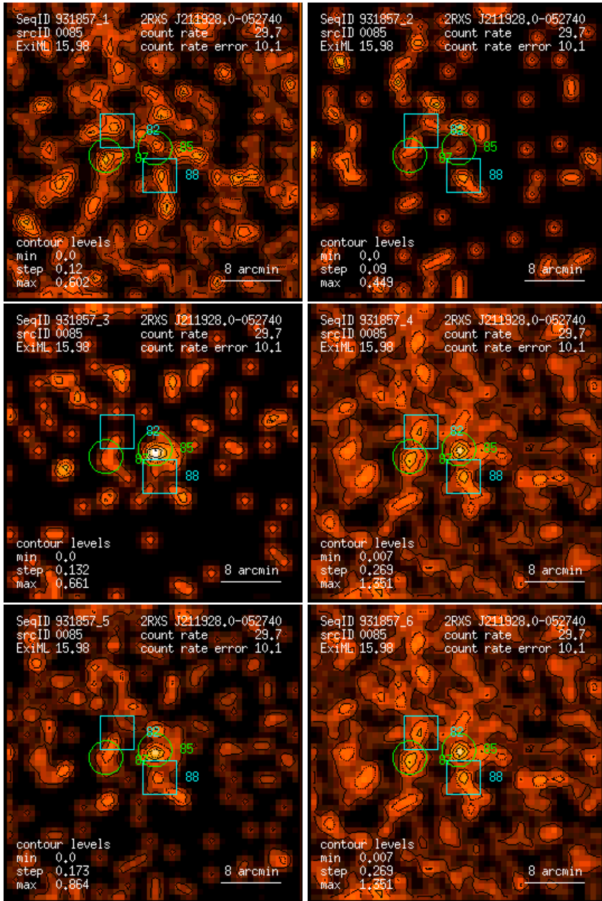
Figure 85: RASS 931857: detection 0085: band rate images, Gaussian filter: (1) PSPC channels 11 – 41, (2) 52 – 90, (3) 91 – 201, (4) 11 – 235, (5) 52 – 201, (6) 11 – 201. Broad band rates in counts/ks. Band rate contour levels in counts/ks/arcmin 2 .
