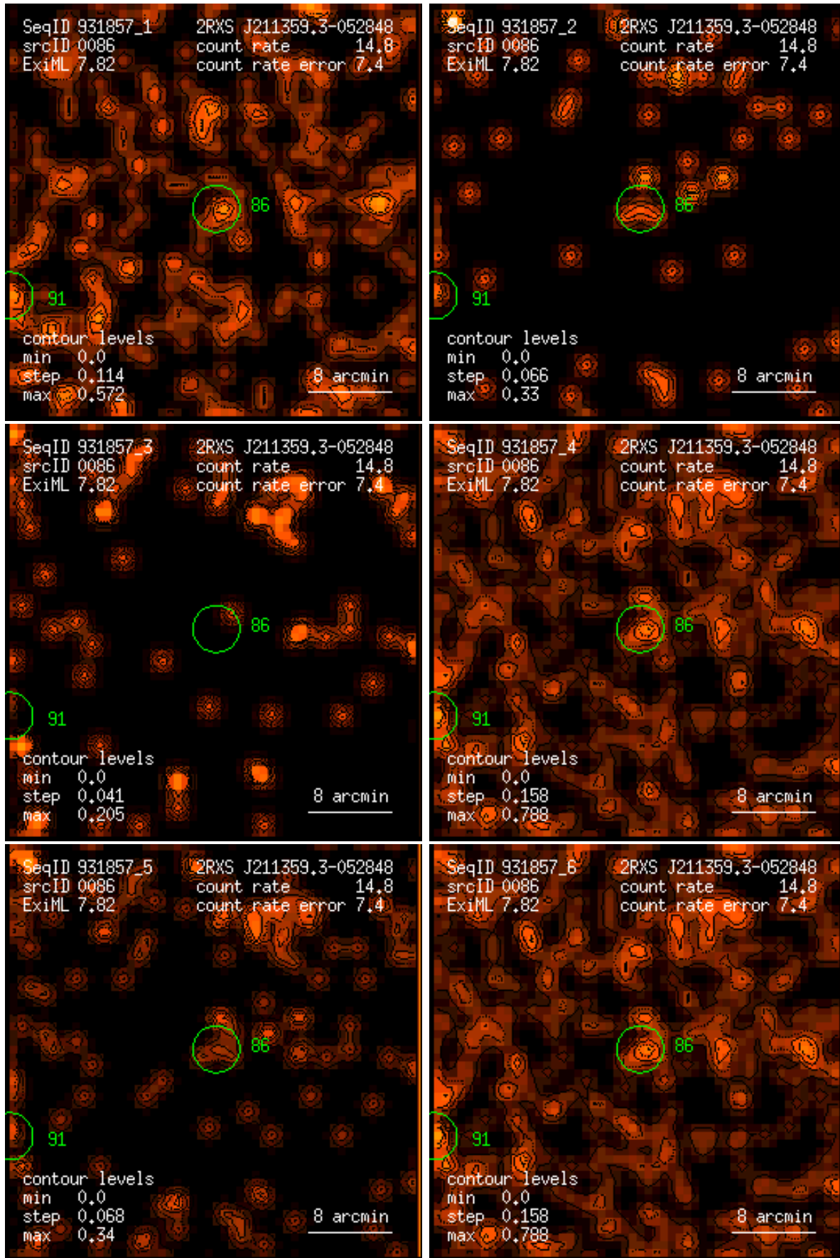
Figure 86: RASS 931857: detection 0086: band rate images, Gaussian filter: (1) PSPC channels 11 – 41, (2) 52 – 90, (3) 91 – 201, (4) 11 – 235, (5) 52 – 201, (6) 11 – 201. Broad band rates in counts/ks. Band rate contour levels in counts/ks/arcmin 2 .
