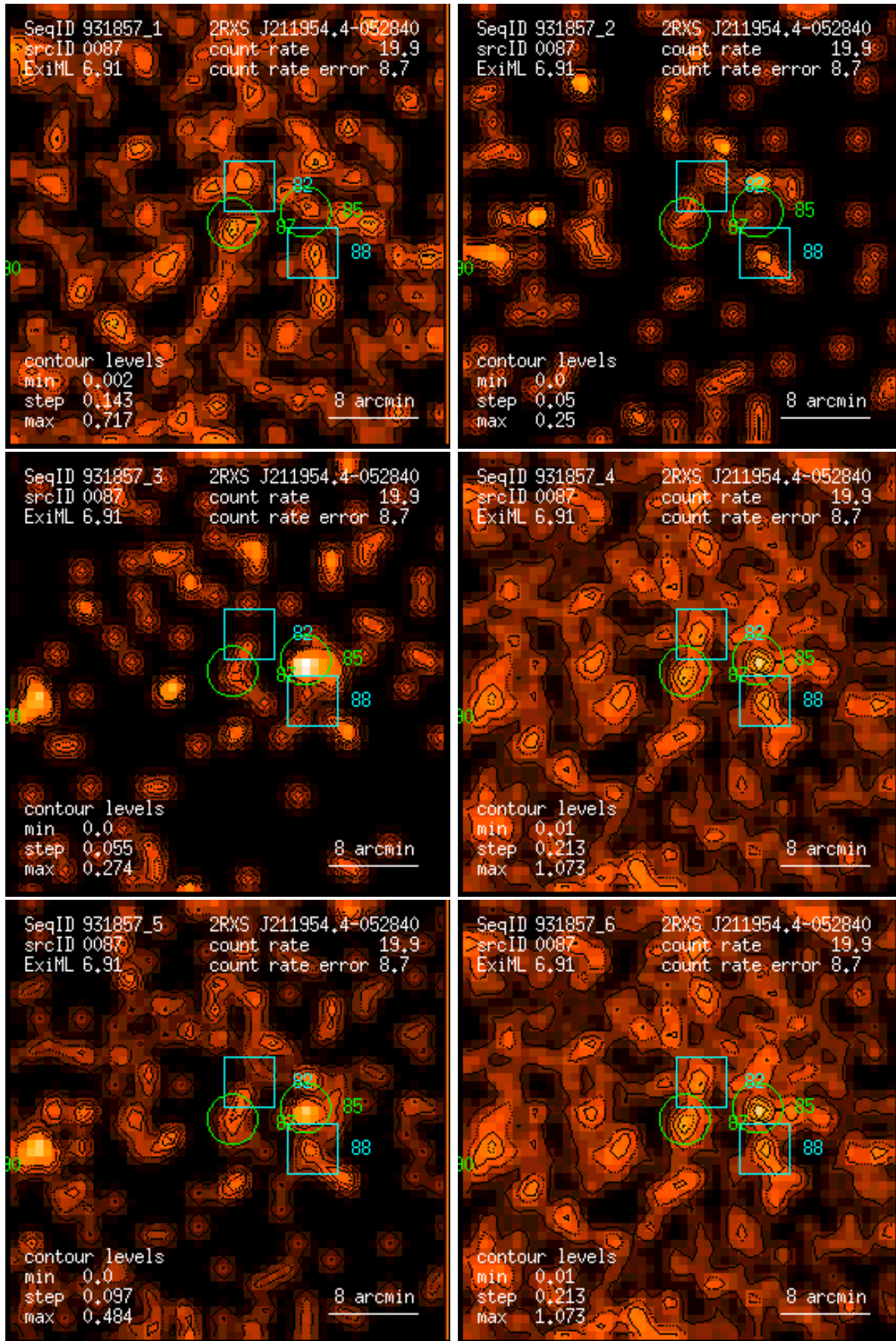
Figure 87: RASS 931857: detection 0087: band rate images, Gaussian filter: (1) PSPC channels 11 – 41, (2) 52 – 90, (3) 91 – 201, (4) 11 – 235, (5) 52 – 201, (6) 11 – 201. Broad band rates in counts/ks. Band rate contour levels in counts/ks/arcmin 2 .
