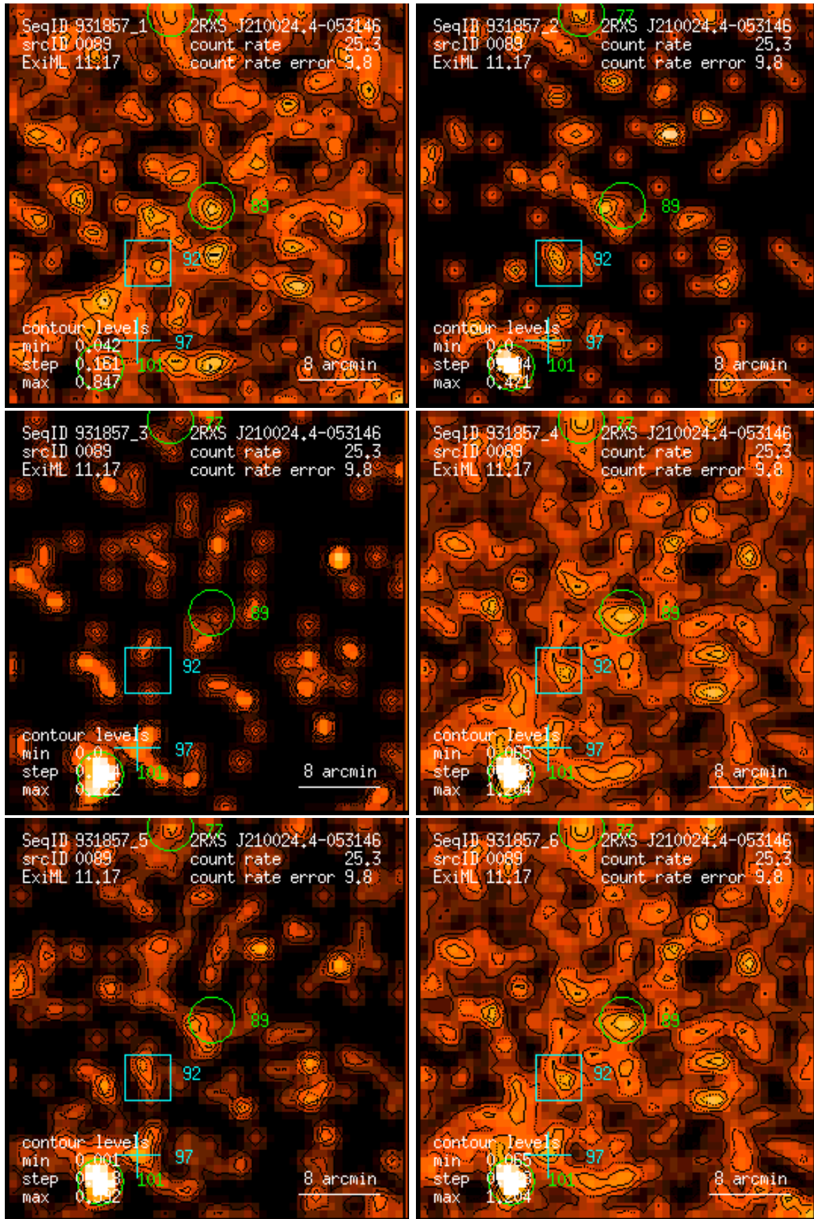
Figure 89: RASS 931857: detection 0089: band rate images, Gaussian filter: (1) PSPC channels 11 – 41, (2) 52 – 90, (3) 91 – 201, (4) 11 – 235, (5) 52 – 201, (6) 11 – 201. Broad band rates in counts/ks. Band rate contour levels in counts/ks/arcmin 2 .
