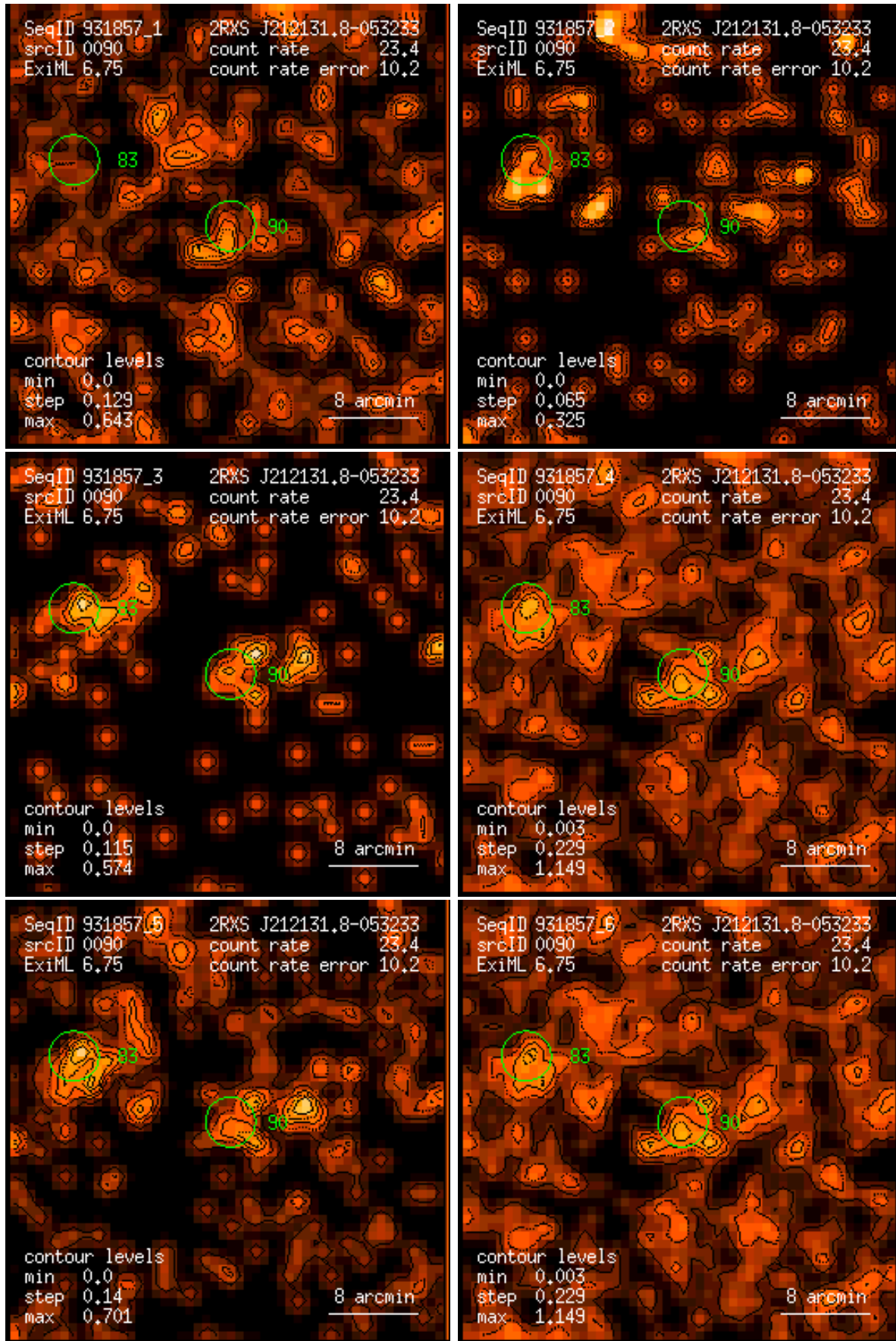
Figure 90: RASS 931857: detection 0090: band rate images, Gaussian filter: (1) PSPP channels 11 – 41, (2) 52 – 90, (3) 91 – 201, (4) 11 – 235, (5) 52 – 201, (6) 11 – 201. Broad band rates in counts/ks. Band rate contour levels in counts/ks/arcmin 2 .
