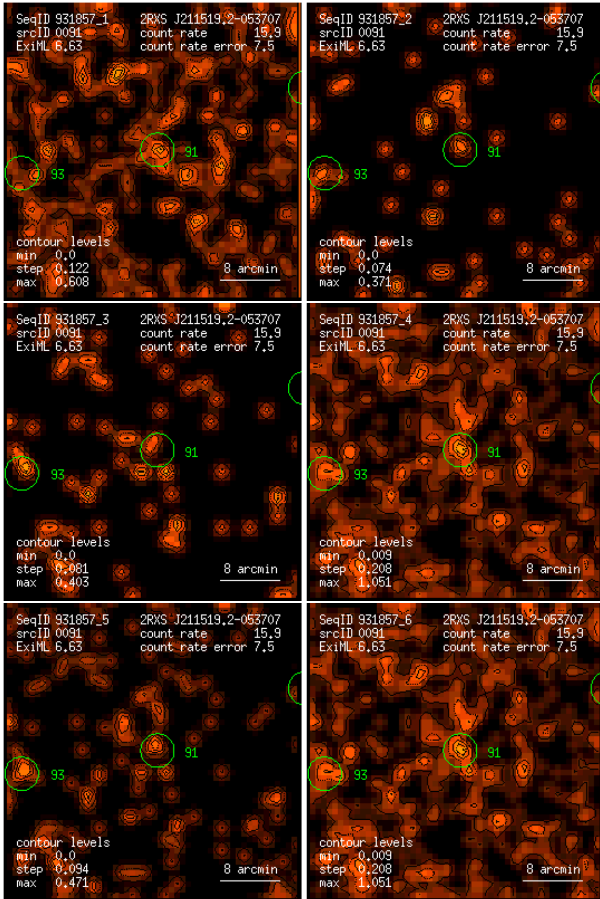
Figure 91: RASS 931857: detection 0091: band rate images, Gaussian filter: (1) PSPC channels 11 – 41, (2) 52 – 90, (3) 91 – 201, (4) 11 – 235, (5) 52 – 201, (6) 11 – 201. Broad band rates in counts/ks. Band rate contour levels in counts/ks/arcmin 2 .
