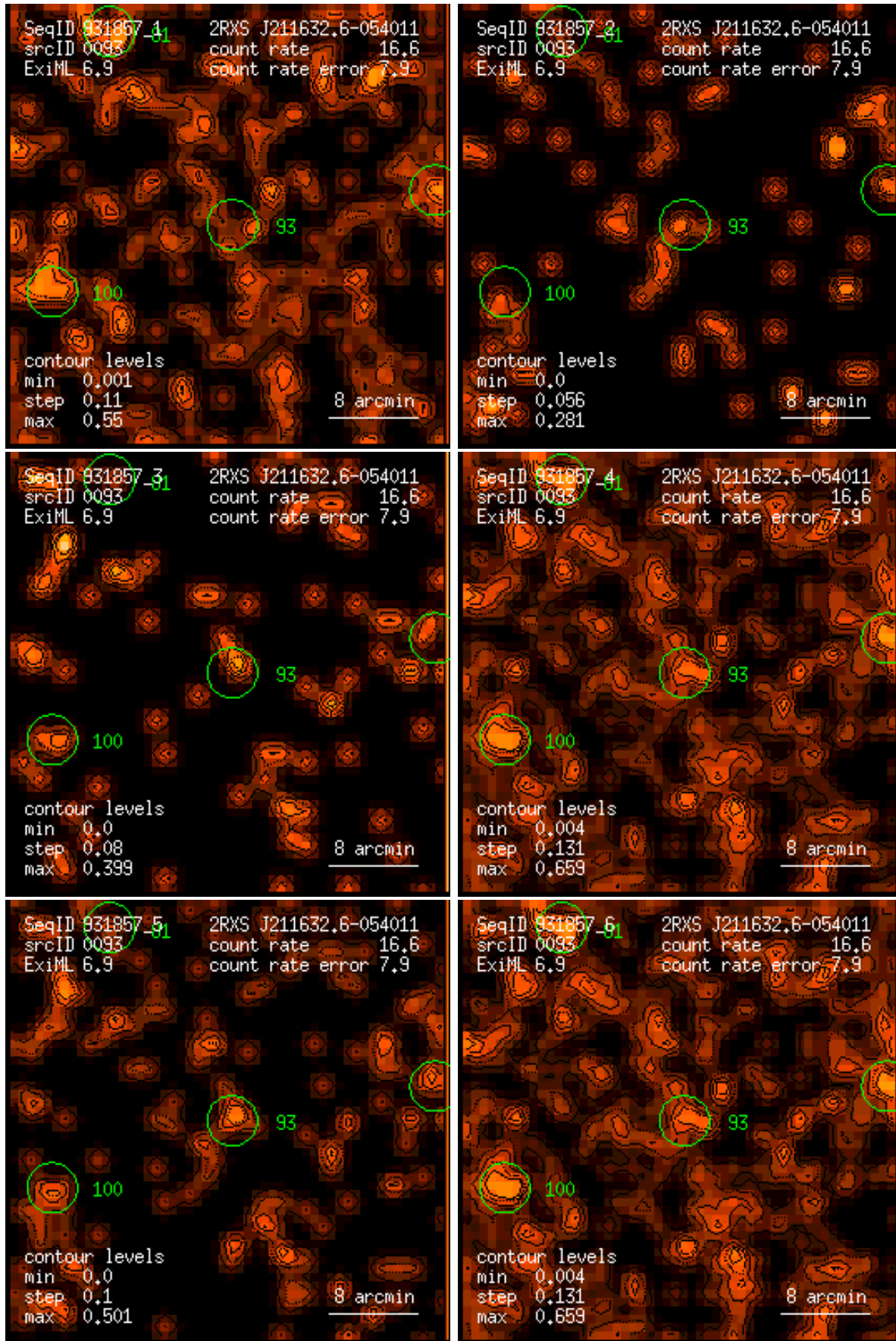
Figure 93: RASS 931857: detection 0093: band rate images, Gaussian filter: (1) PSPC channels 11 – 41, (2) 52 – 90, (3) 91 – 201, (4) 11 – 235, (5) 52 – 201, (6) 11 – 201. Broad band rates in counts/ks. Band rate contour levels in counts/ks/arcmin 2 .
