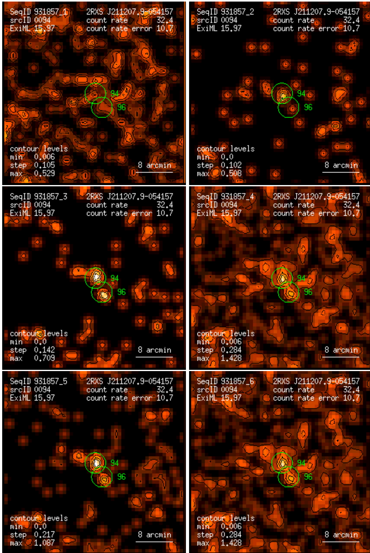
Figure 94: RASS 931857: detection 0094: band rate images, Gaussian filter: (1) PSPC channels 11 – 41, (2) 52 – 90, (3) 91 – 201, (4) 11 – 235, (5) 52 – 201, (6) 11 – 201. Broad band rates in counts/ks. Band rate contour levels in counts/ks/arcmin 2 .
