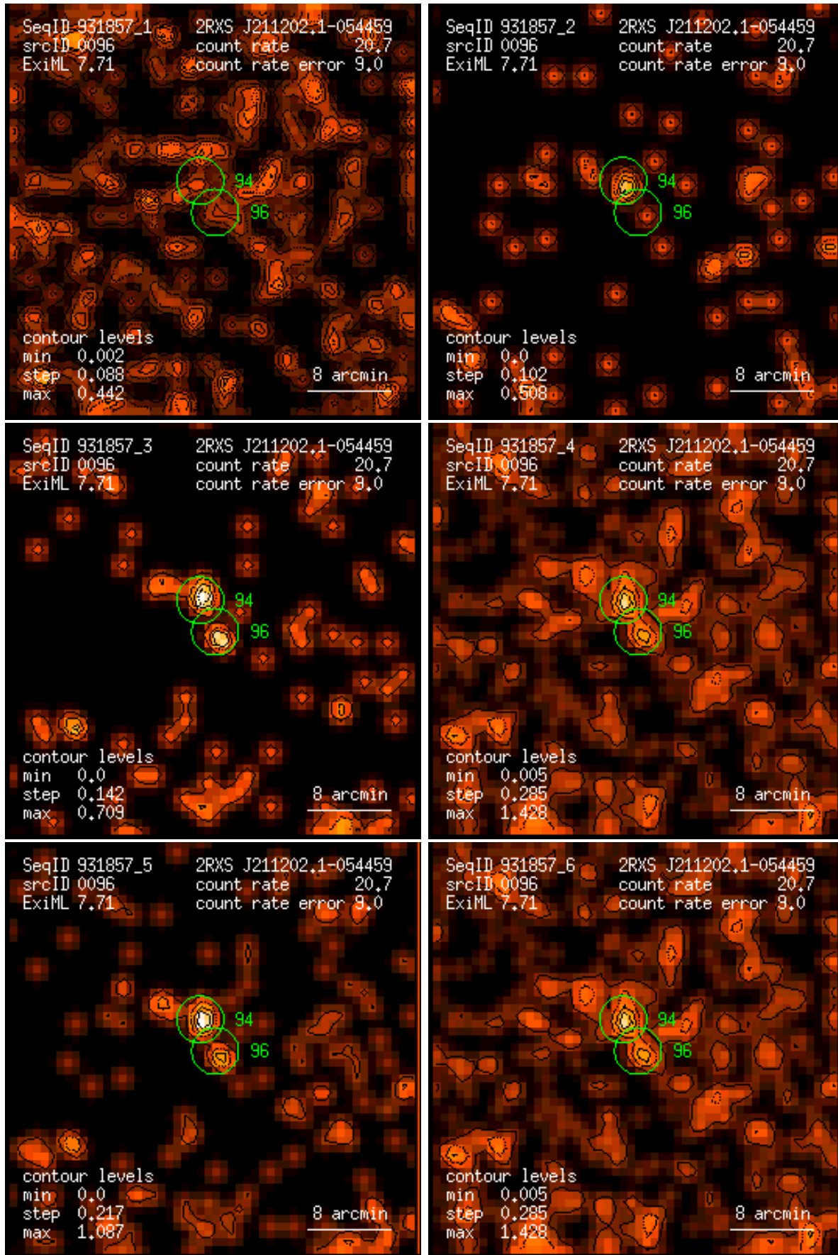
Figure 96: RASS 931857: detection 0096: band rate images, Gaussian filter: (1) PSPC channels 11 – 41, (2) 52 – 90, (3) 91 – 201, (4) 11 – 235, (5) 52 – 201, (6) 11 – 201. Broad band rates in counts/ks. Band rate contour levels in counts/ks/arcmin 2 .
