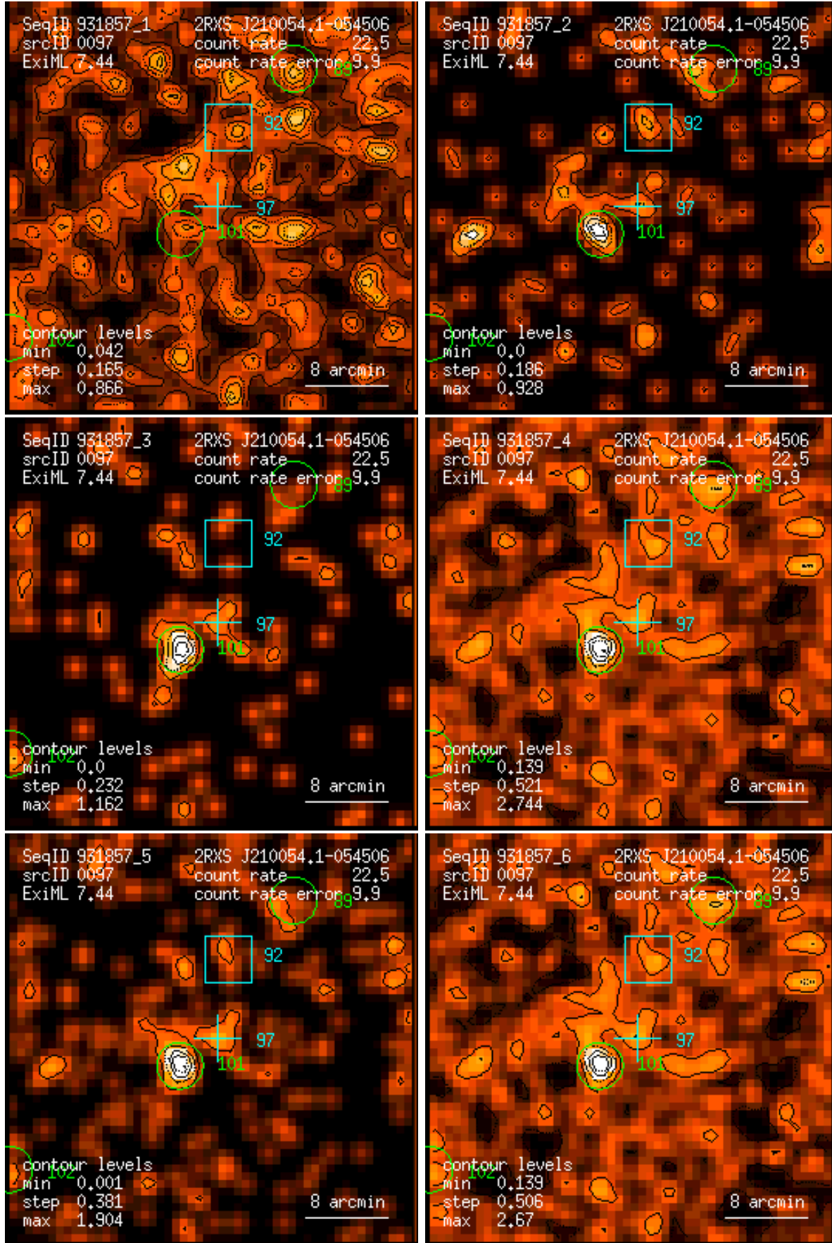
Figure 97: RASS 931857: detection 0097: band rate images, Gaussian filter: (1) PSPC channels 11 – 41, (2) 52 – 90, (3) 91 – 201, (4) 11 – 235, (5) 52 – 201, (6) 11 – 201. Broad band rates in counts/ks. Band rate contour levels in counts/ks/arcmin 2 .
