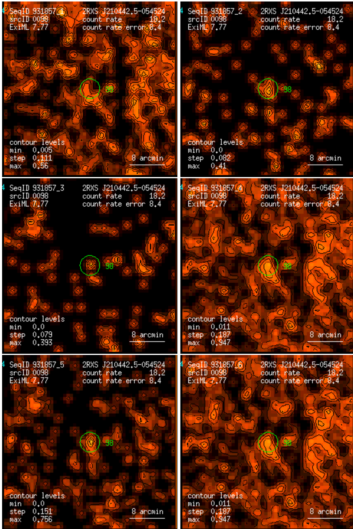
Figure 98: RASS 931857: detection 0098: band rate images, Gaussian filter: (1) PSPC channels 11 – 41, (2) 52 – 90, (3) 91 – 201, (4) 11 – 235, (5) 52 – 201, (6) 11 – 201. Broad band rates in counts/ks. Band rate contour levels in counts/ks/arcmin 2 .
