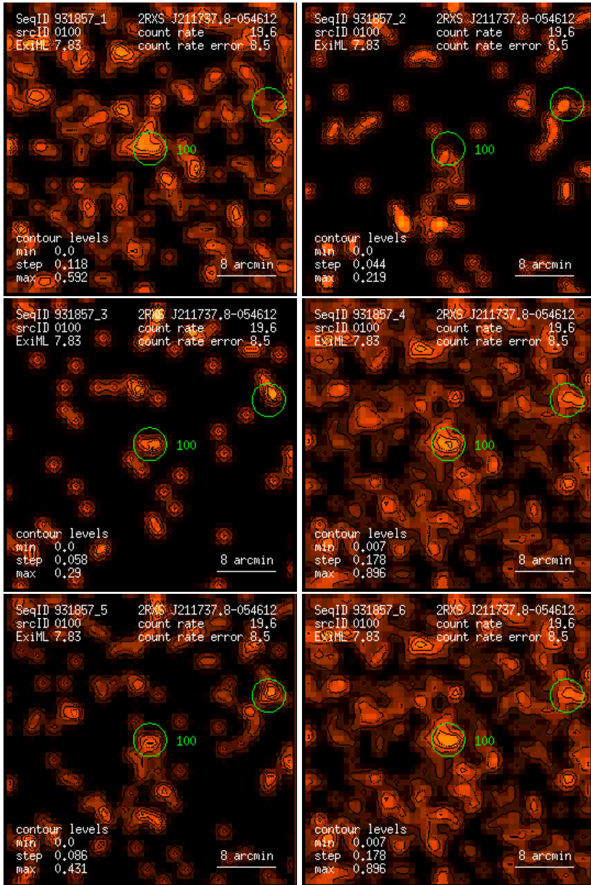
Figure 100: RASS 931857: detection 0100: band rate images, Gaussian filter: (1) PSPC channels 11 – 41, (2) 52 – 90, (3) 91 – 201, (4) 11 – 235, (5) 52 – 201, (6) 11 – 201. Broad band rates in counts/ks. Band rate contour levels in counts/ks/arcmin 2 .
