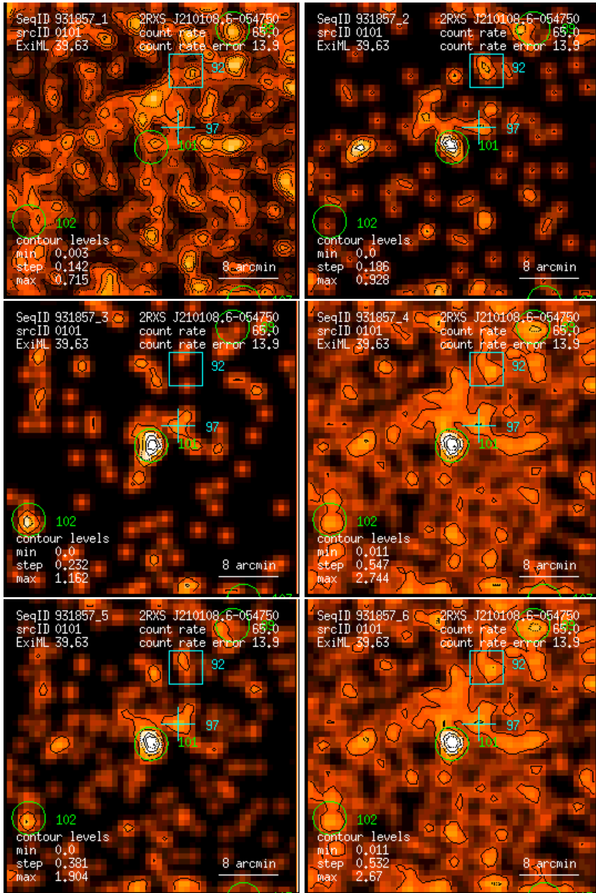
Figure 101: RASS 931857: detection 0101: band rate images, Gaussian filter: (1) PSPC channels 11 – 41, (2) 52 – 90, (3) 91 – 201, (4) 11 – 235, (5) 52 – 201, (6) 11 – 201. Broad band rates in counts/ks. Band rate contour levels in counts/ks/arcmin 2 .
