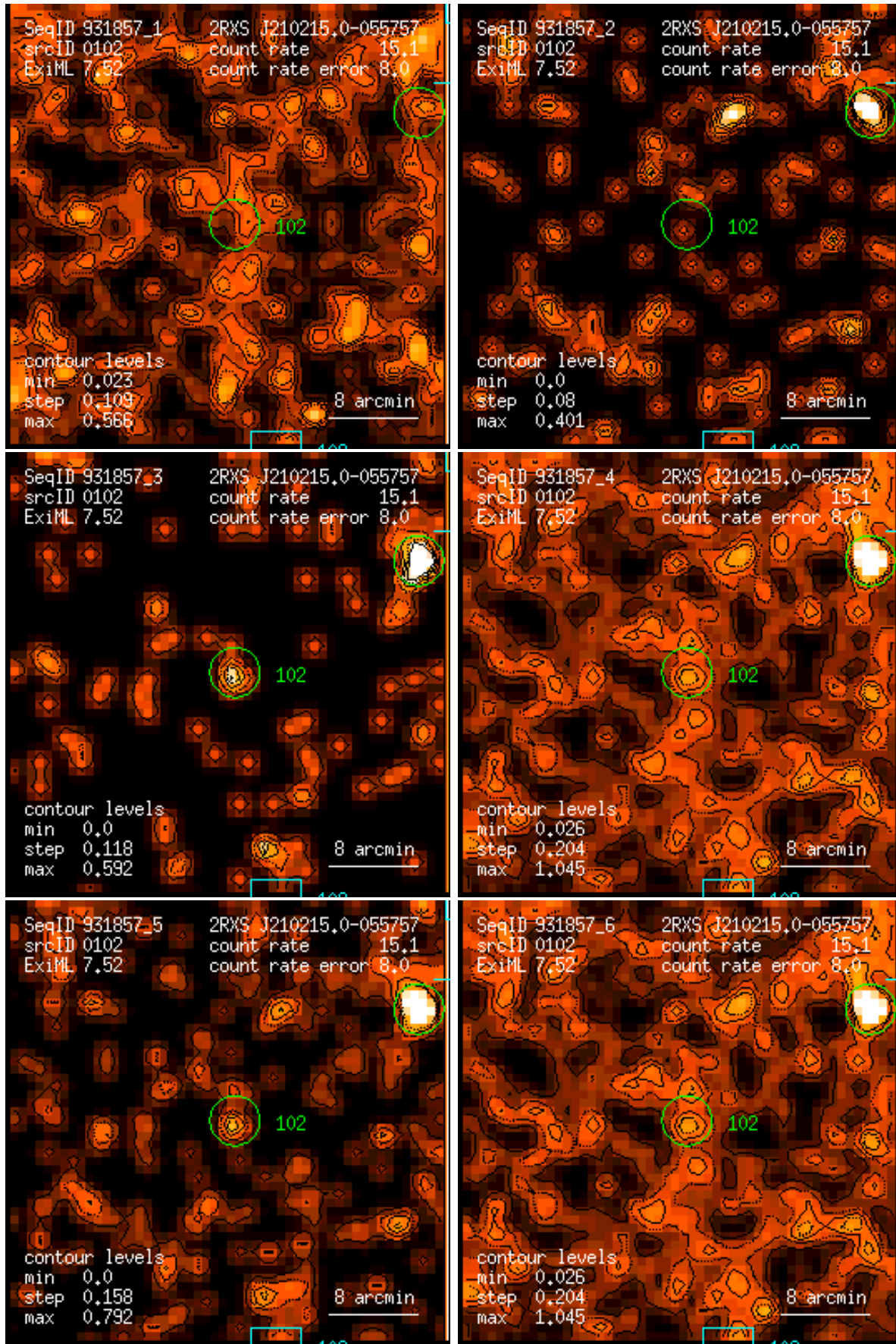
Figure 102: RASS 931857: detection 0102: band rate images, Gaussian filter: (1) PSPC channels 11 – 41, (2) 52 – 90, (3) 91 – 201, (4) 11 – 235, (5) 52 – 201, (6) 11 – 201. Broad band rates in counts/ks. Band rate contour levels in counts/ks/arcmin 2 .
