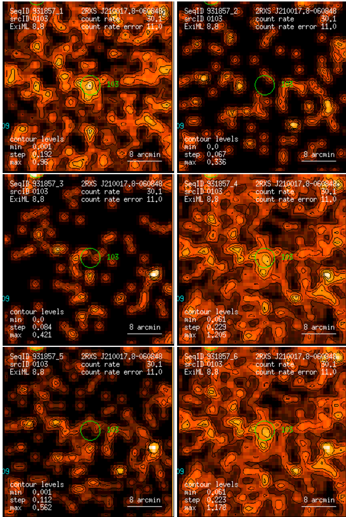
Figure 103: RASS 931857: detection 0103: band rate images, Gaussian filter: (1) PSPC channels 11 – 41, (2) 52 – 90, (3) 91 – 201, (4) 11 – 235, (5) 52 – 201, (6) 11 – 201. Broad band rates in counts/ks. Band rate contour levels in counts/ks/arcmin 2 .
