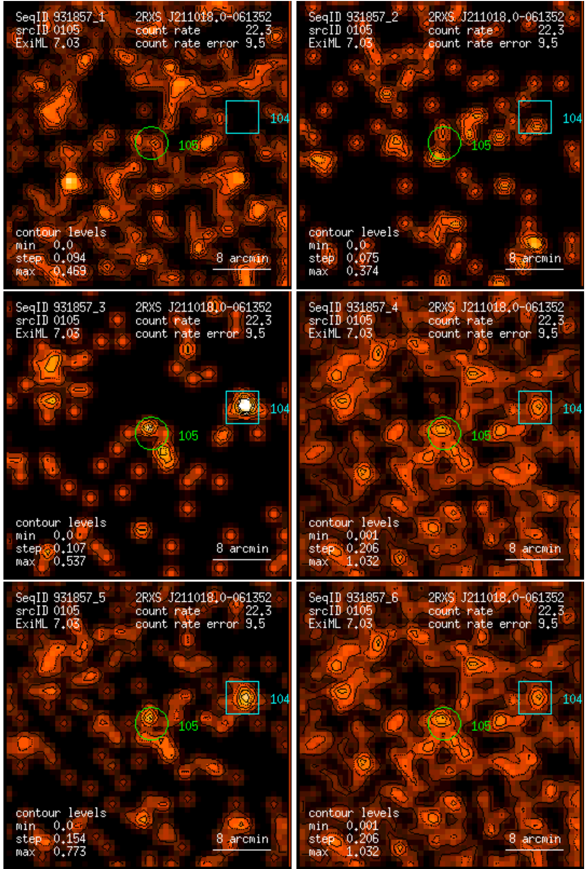
Figure 105: RASS 931857: detection 0105: band rate images, Gaussian filter: (1) PSPC channels 11 – 41, (2) 52 – 90, (3) 91 – 201, (4) 11 – 235, (5) 52 – 201, (6) 11 – 201. Broad band rates in counts/ks. Band rate contour levels in counts/ks/arcmin 2 .
