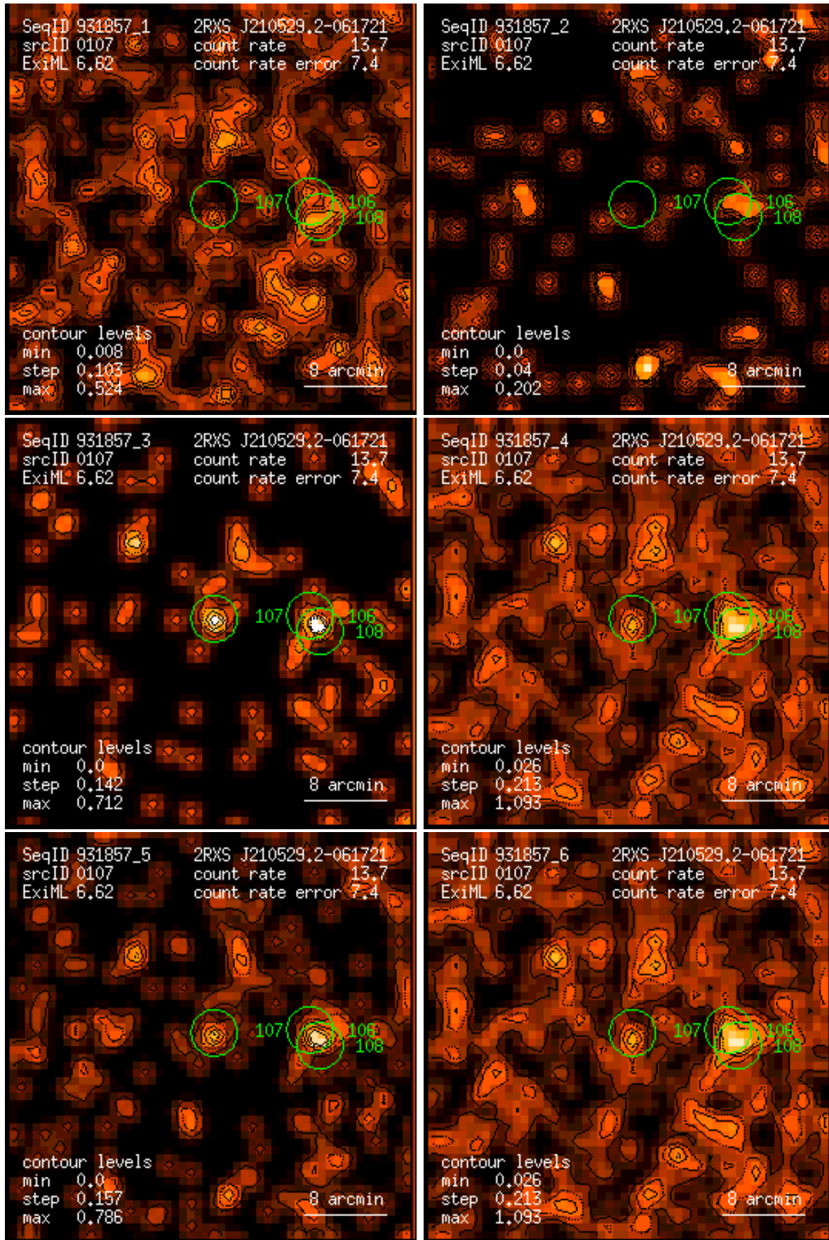
Figure 107: RASS 931857: detection 0107: band rate images, Gaussian filter: (1) PSPC channels 11 – 41, (2) 52 – 90, (3) 91 – 201, (4) 11 – 235, (5) 52 – 201, (6) 11 – 201. Broad band rates in counts/ks. Band rate contour levels in counts/ks/arcmin 2 .
