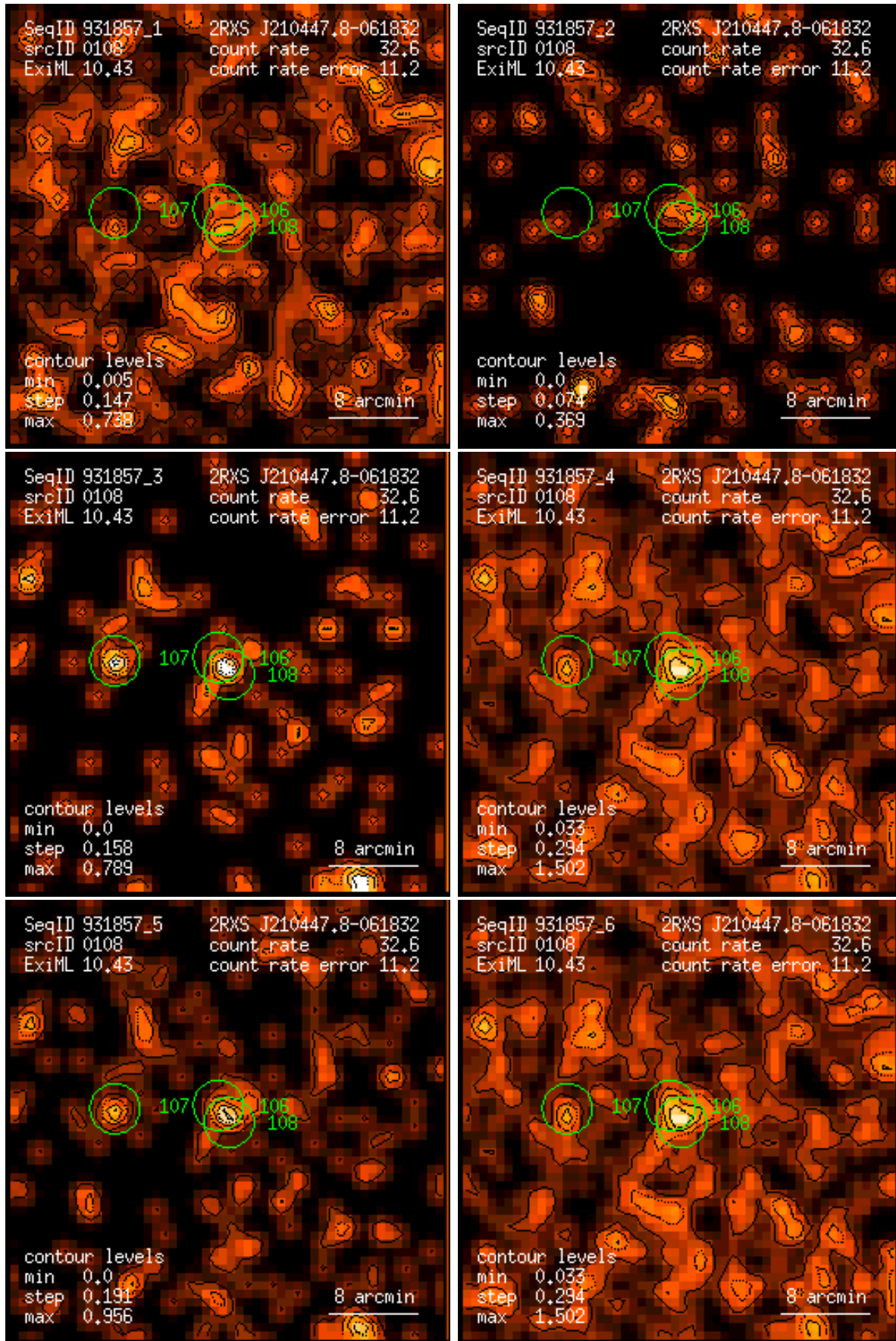
Figure 108: RASS 931857: detection 0108: band rate images, Gaussian filter: (1) PSPC channels 11 – 41, (2) 52 – 90, (3) 91 – 201, (4) 11 – 235, (5) 52 – 201, (6) 11 – 201. Broad band rates in counts/ks. Band rate contour levels in counts/ks/arcmin 2 .
