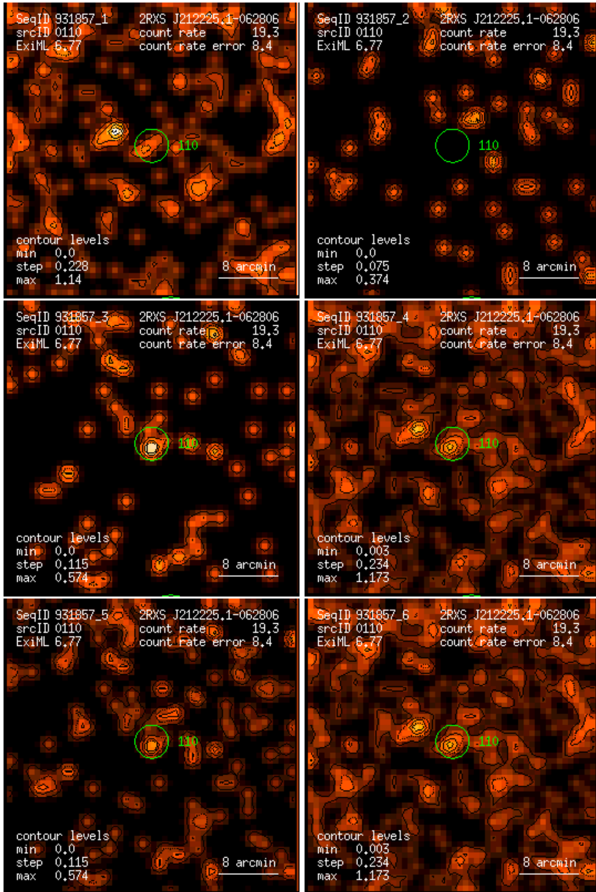
Figure 110: RASS 931857: detection 0110: band rate images, Gaussian filter: (1) PSPC channels 11 – 41, (2) 52 – 90, (3) 91 – 201, (4) 11 – 235, (5) 52 – 201, (6) 11 – 201. Broad band rates in counts/ks. Band rate contour levels in counts/ks/arcmin 2 .
